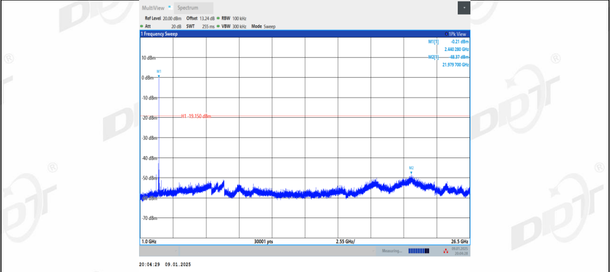
BLE_2M_Right side_2440_0~Reference
