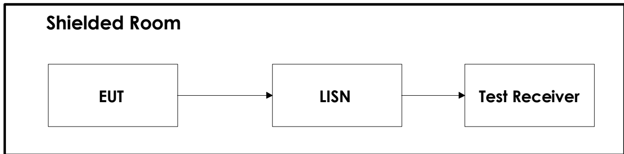
Test Set-Up 5
