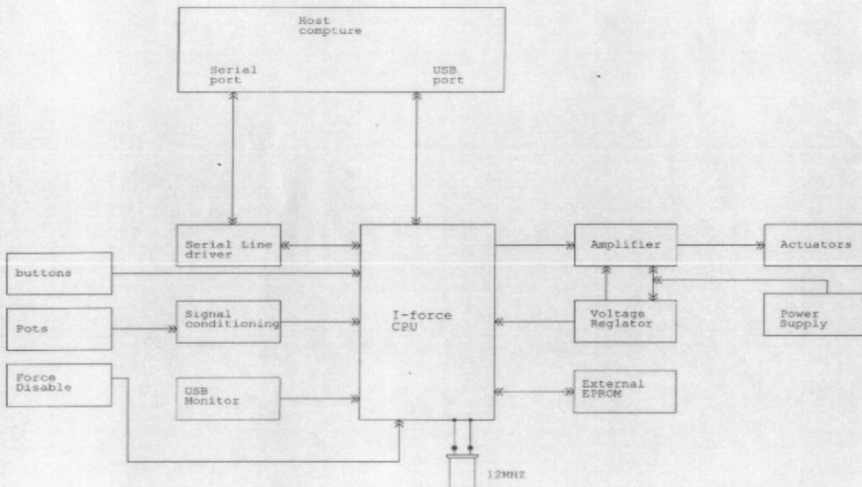
Force feed back game device block diagram
