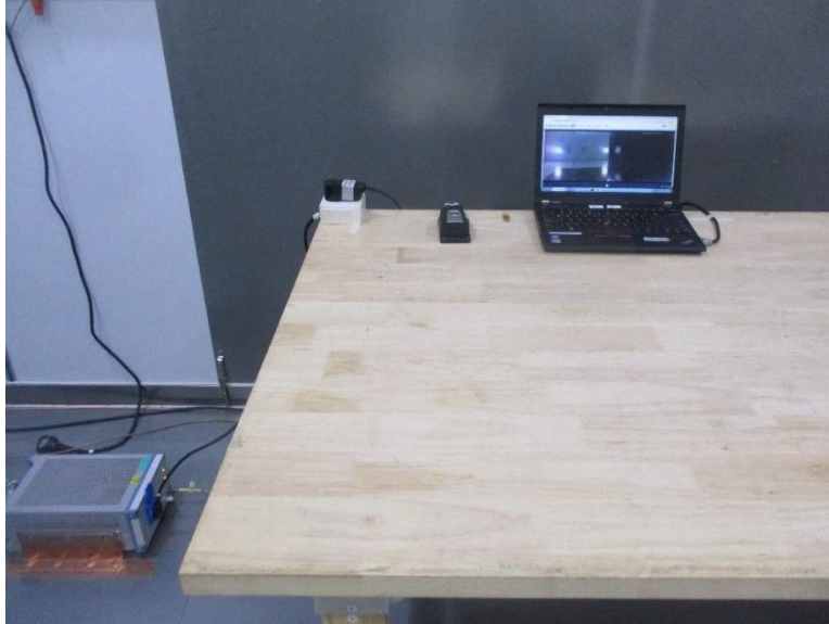
Conducted Disturbance Emissions on AC mains
