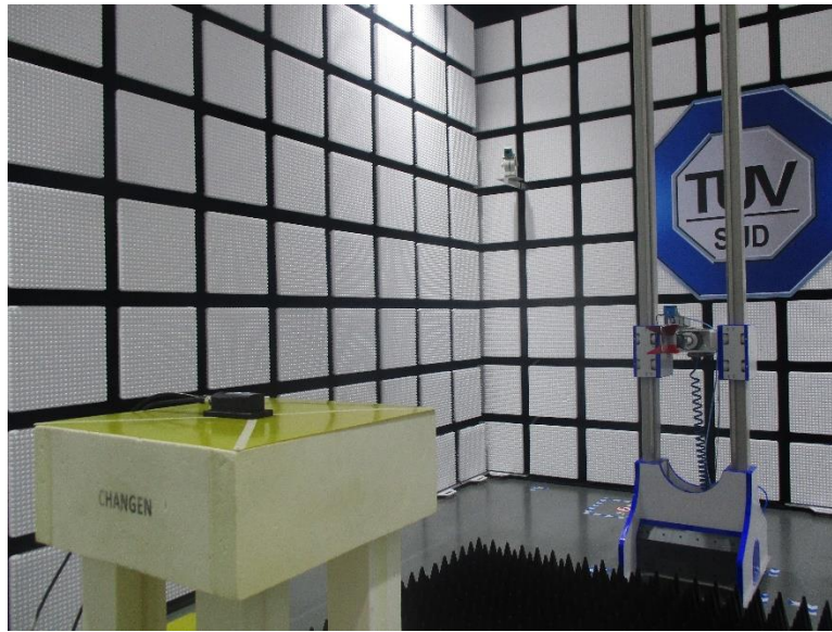
Radiated Spurious emission 1GHz-18GHz
