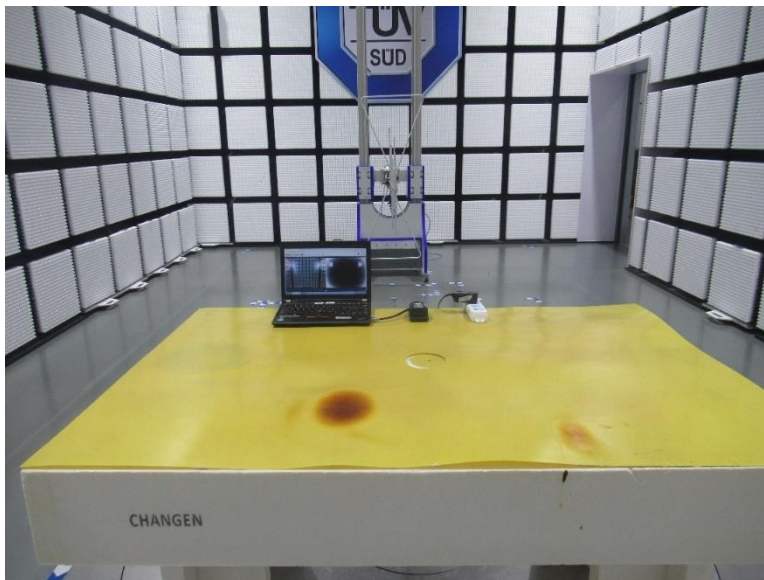
Radiated Spurious emission 30MHz-1GHz
