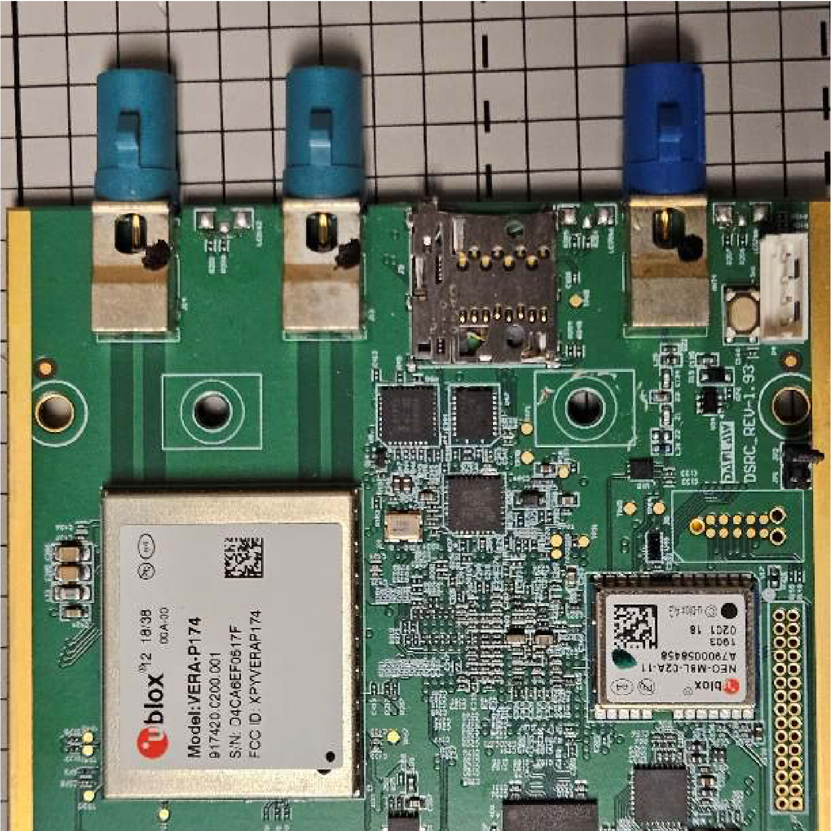
DSRC RADIO BOARD (PRECERT MODULE)
