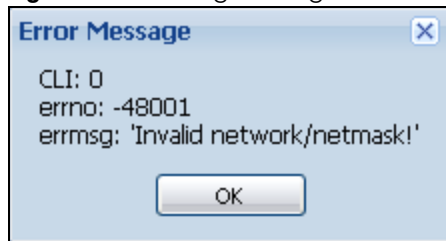
Figure 17 Warning Message
