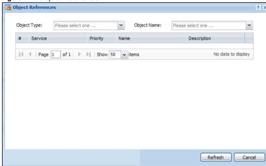
Figure 14 Object Reference
