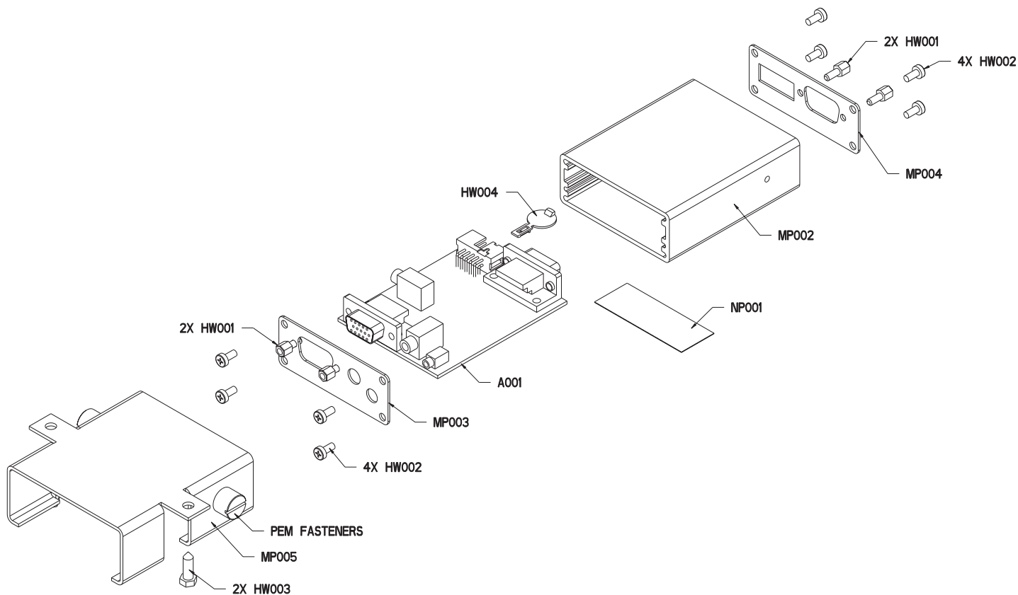
HANDHELD CONTROL UNIT JUNCTION BOX EXPLODED VIEW
