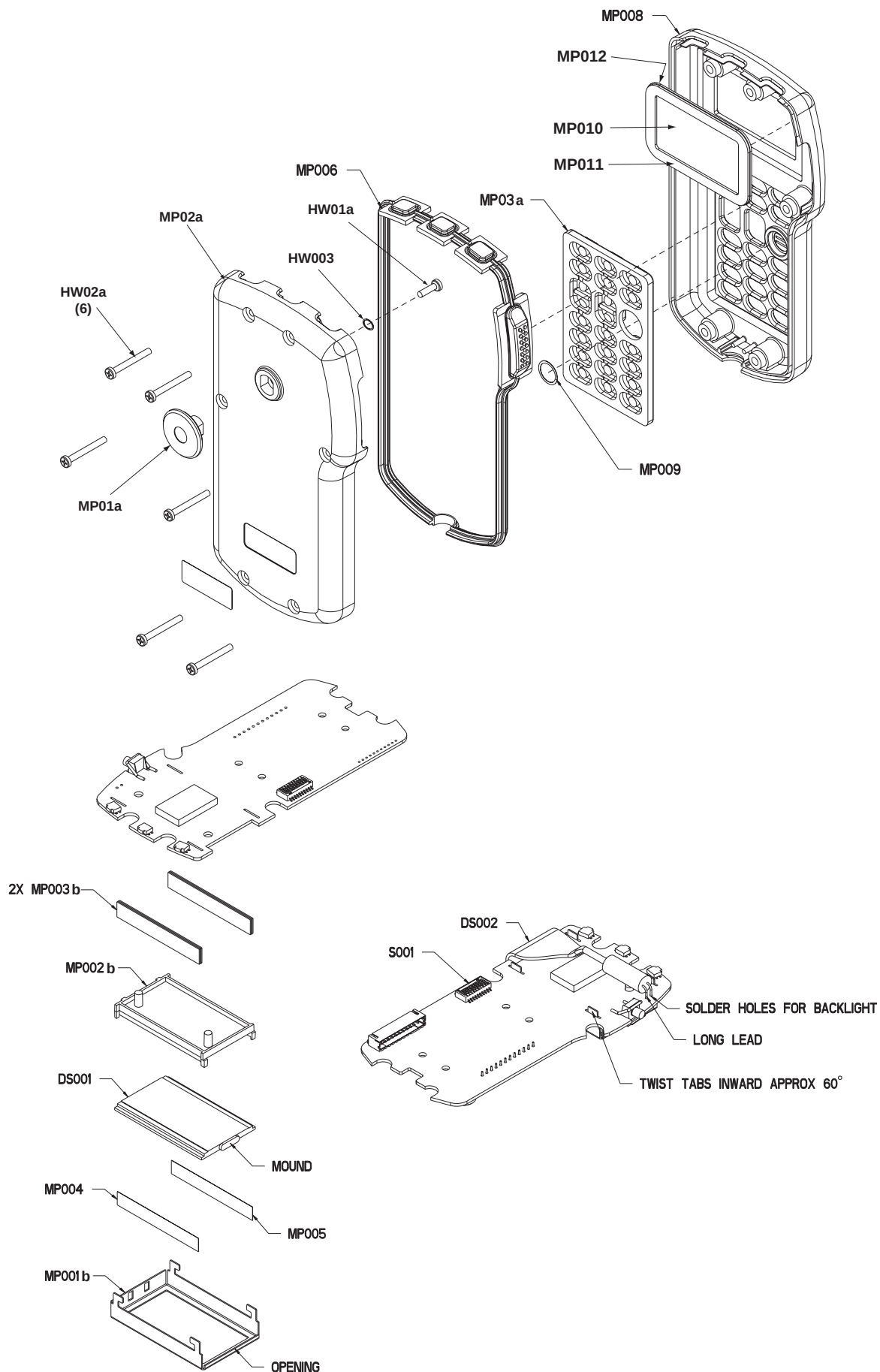
HANDHELD CONTROL UNIT EXPLODED VIEW (PART 2 OF 2)
