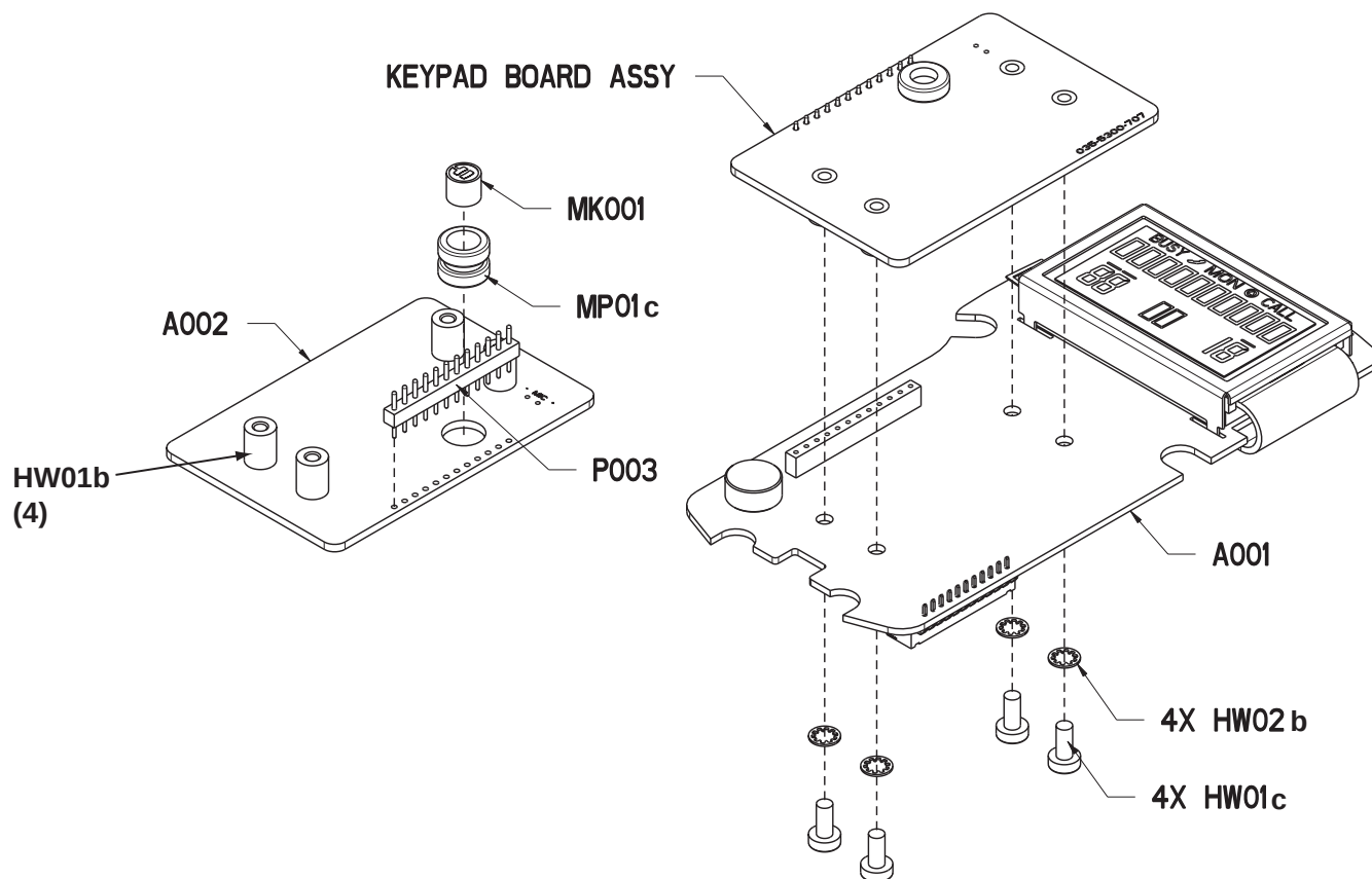
HANDHELD CONTROL UNIT EXPLODED VIEW (PART 1 OF 2)
