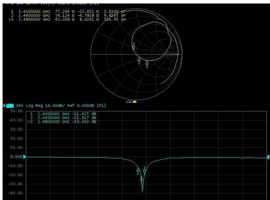
Return Loss
