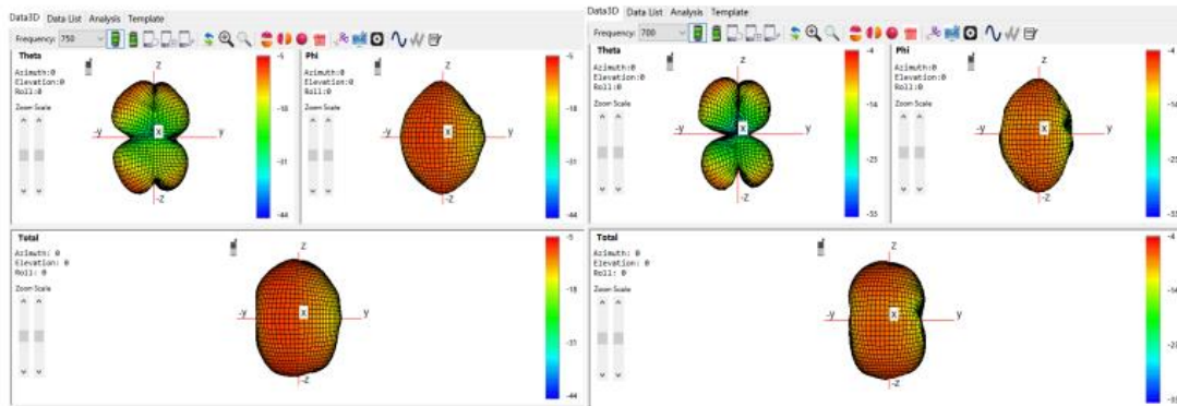
698-960MHz 3D and 2D Radiation Patterns:
