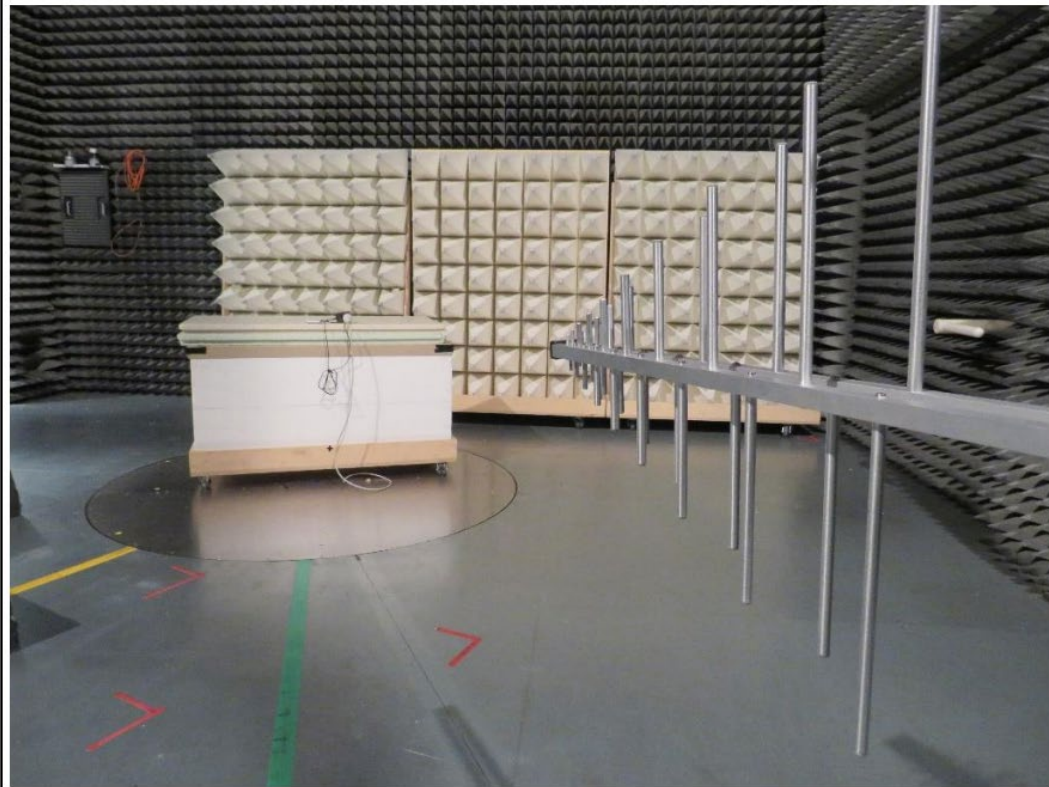
Radiated test setup below 1 GHz
