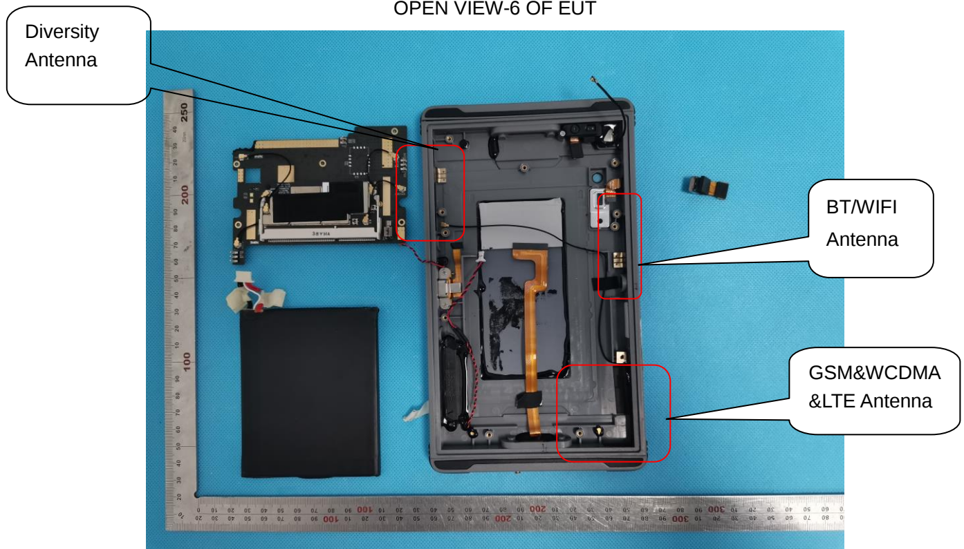
OPEN VIEW-6 OF EUT
