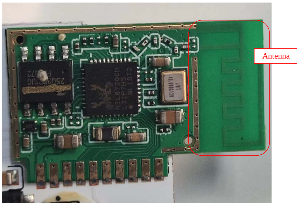
FIGURE 17 DOWNLIGHT (M/N: CFIXCNLR6C1) CHIP&CRYSTAL ON BOARD
