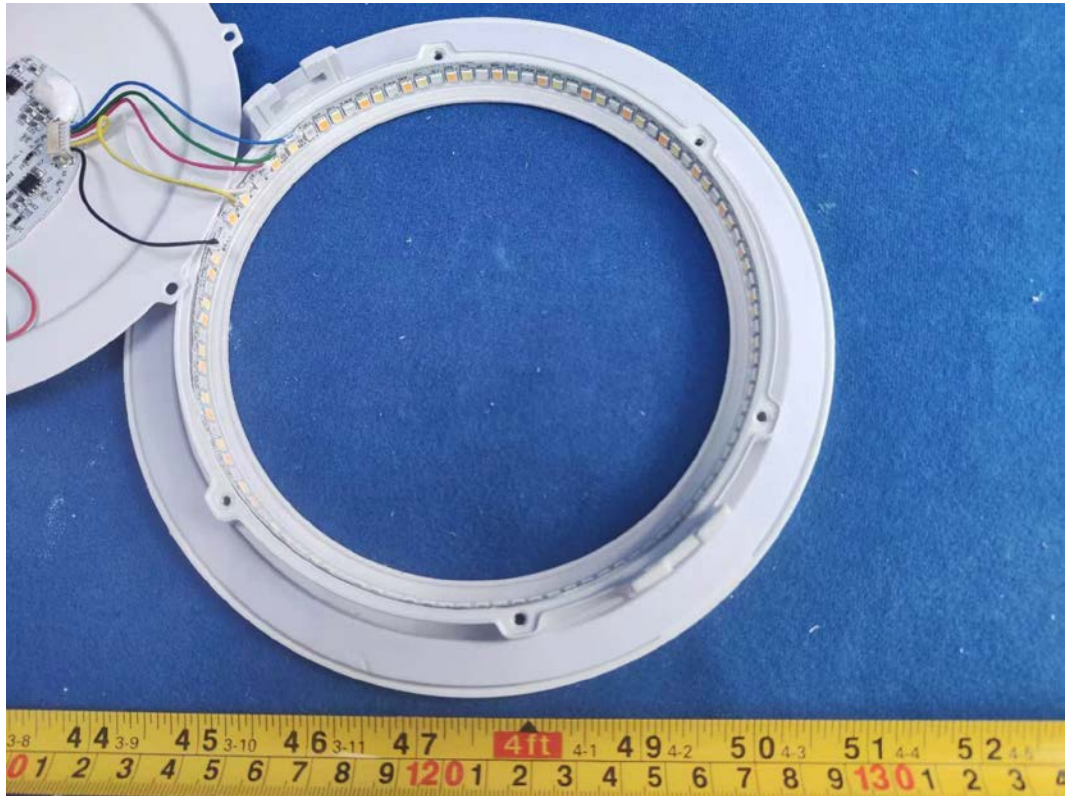
FIGURE 11 DOWNLIGHT (M/N: CFIXCNLR6CRVD) LED
