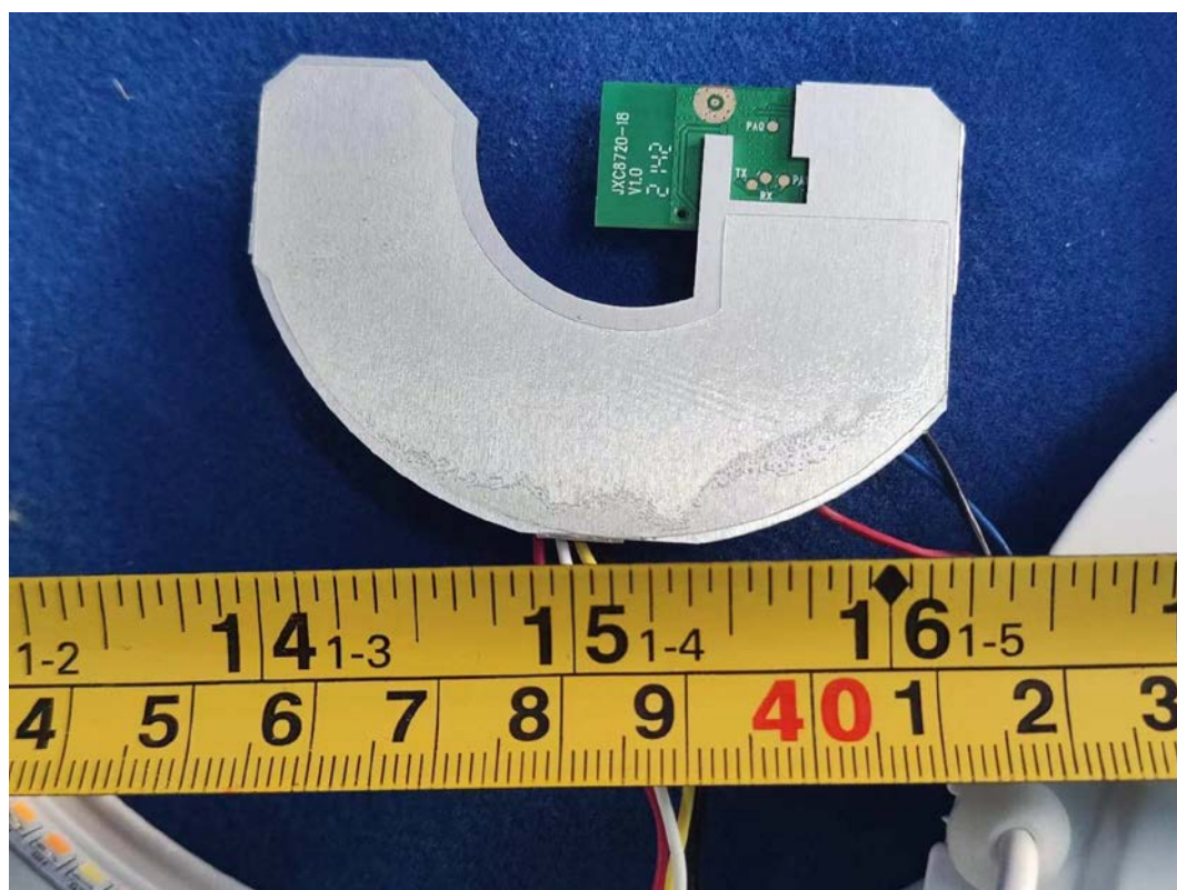
FIGURE 16 DOWNLIGHT (M/N: CFIXCNLR6C1) MAIN BOARD (SOLDERED SIDE)
