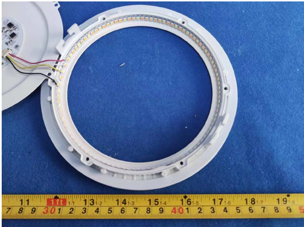
FIGURE 18 DOWNLIGHT (M/N: CFIXCNLR6C1) LED
