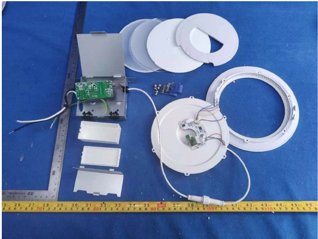
FIGURE 5 DOWNLIGHT (M/N: CFIXCNLR6CRVD) COVER REMOVED
