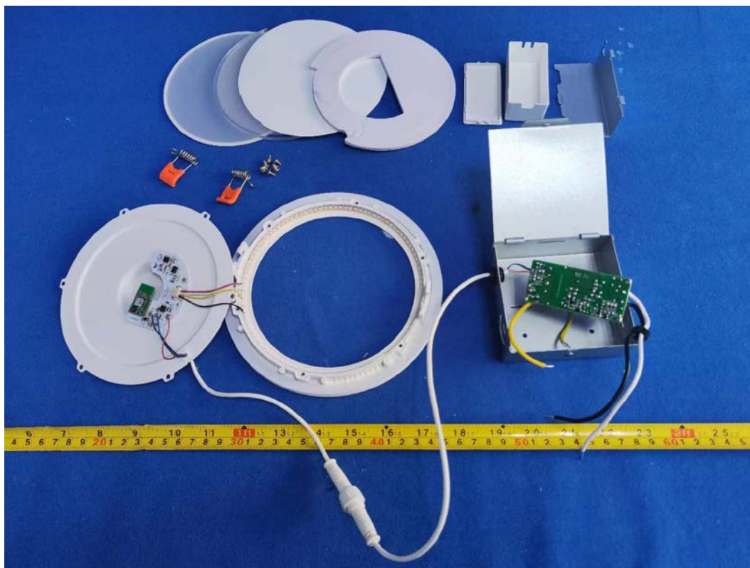
FIGURE 12 DOWNLIGHT (M/N: CFIXCNLR6C1) COVER REMOVED
