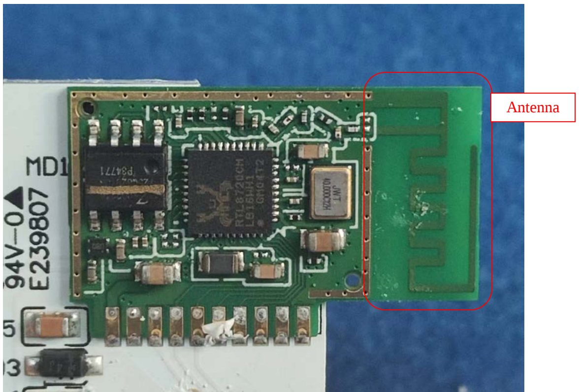
FIGURE 10 DOWNLIGHT (M/N: CFIXCNLR6CRVD) CHIP&CRYSTAL ON BOARD
