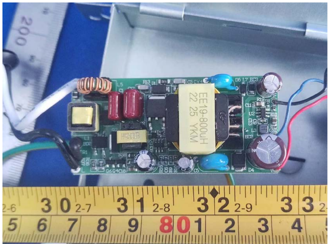
FIGURE 6 DOWNLIGHT (M/N: CFIXCNLR6CRVD) POWER BOARD (COMPONENT SIDE)
