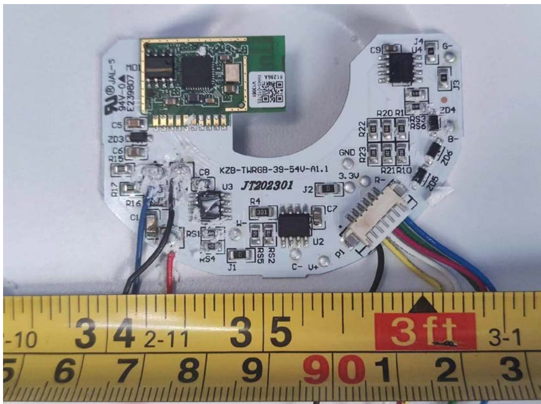
FIGURE 8 DOWNLIGHT (M/N: CFIXCNLR6CRVD) MAIN BOARD (COMPONENT SIDE)
