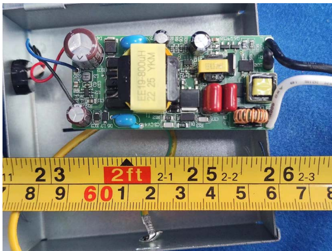
FIGURE 13 DOWNLIGHT (M/N: CFIXCNLR6C1) POWER BOARD (COMPONENT SIDE)
