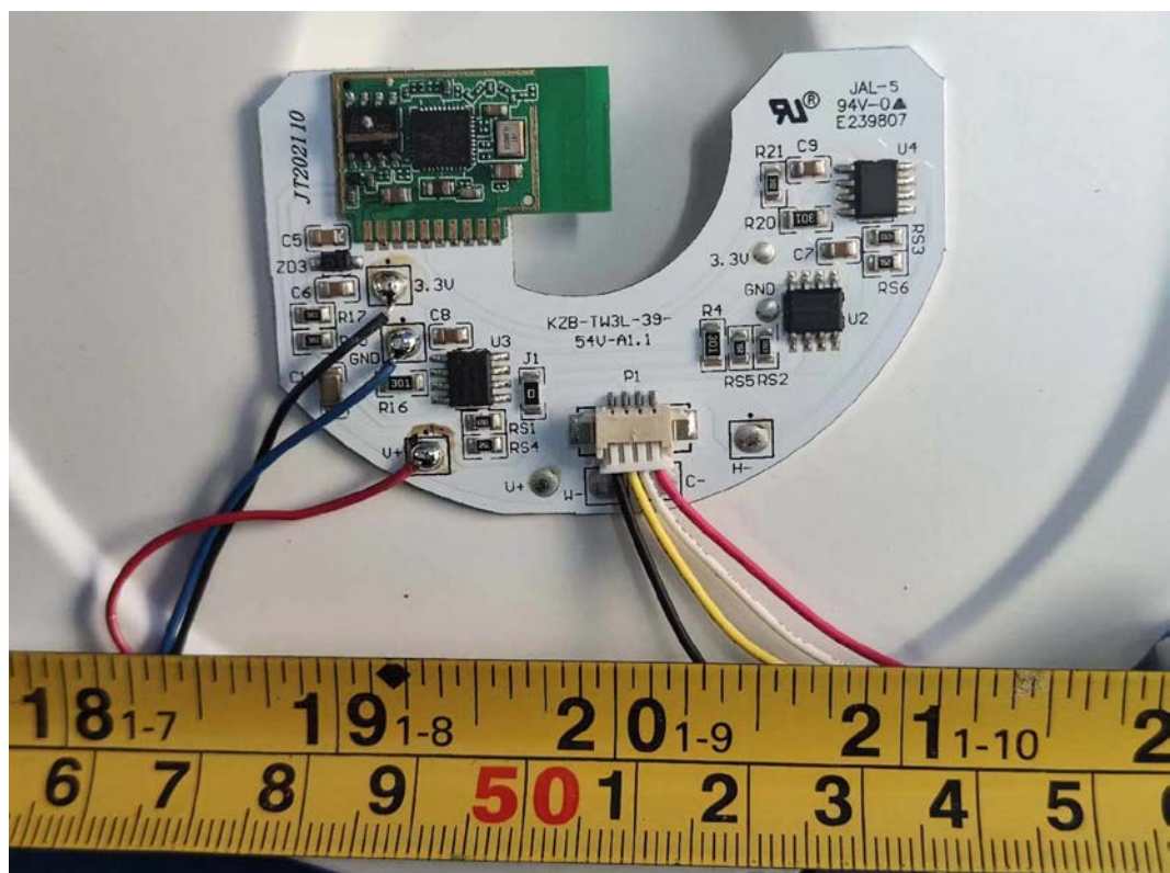
FIGURE 15 DOWNLIGHT (M/N: CFIXCNLR6C1) MAIN BOARD (COMPONENT SIDE)
