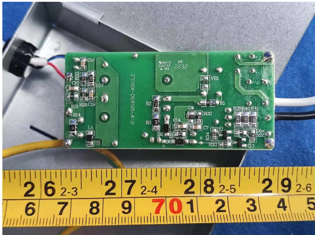
FIGURE 14 DOWNLIGHT (M/N: CFIXCNLR6C1) POWER BOARD (SOLDERED SIDE)
