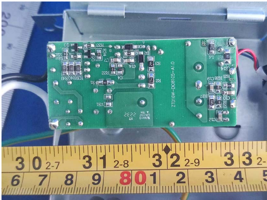
FIGURE 7 DOWNLIGHT (M/N: CFIXCNLR6CRVD) POWER BOARD (SOLDERED SIDE)
