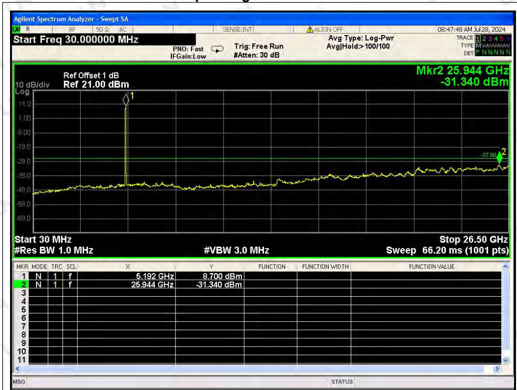
Spurious_Emission_NVNT_802_11a_5180_20M
