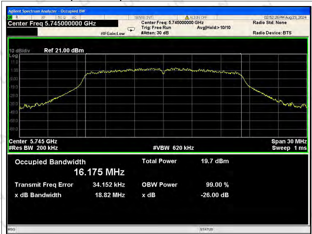
802.11a_ANT1_5745_6Mbps_OBW
