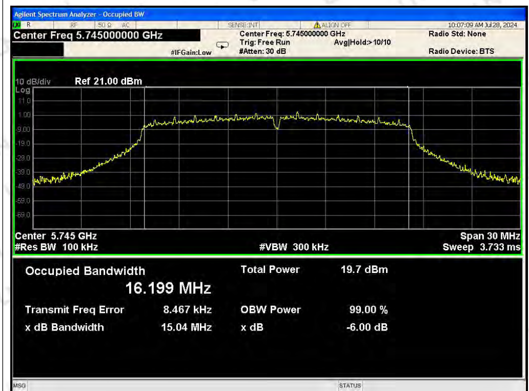
802.11n20_ANT1_5745_MCS0_OBW
