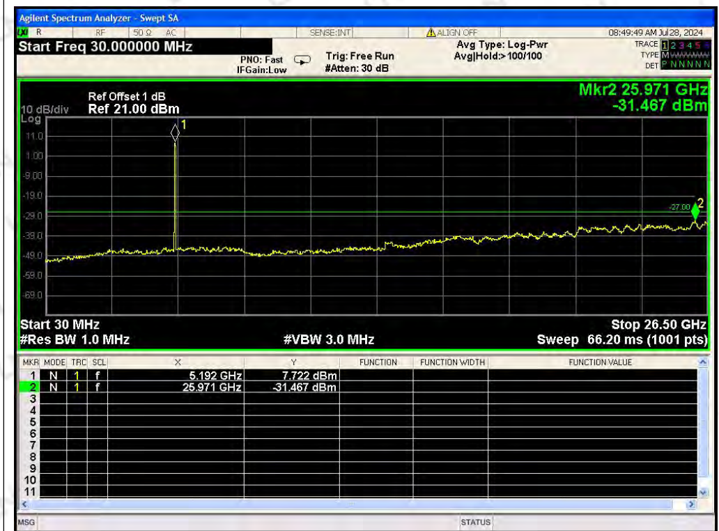
Spurious_Emission_NVNT_802_11a_5200_20M
