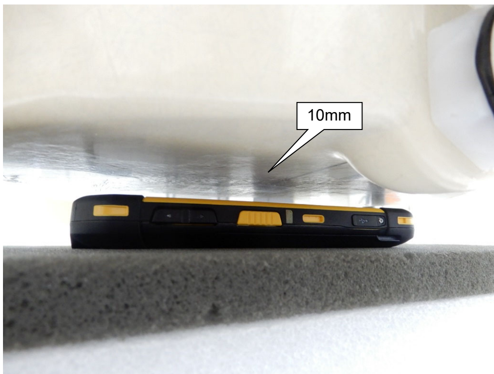
EUT Front_10mm
