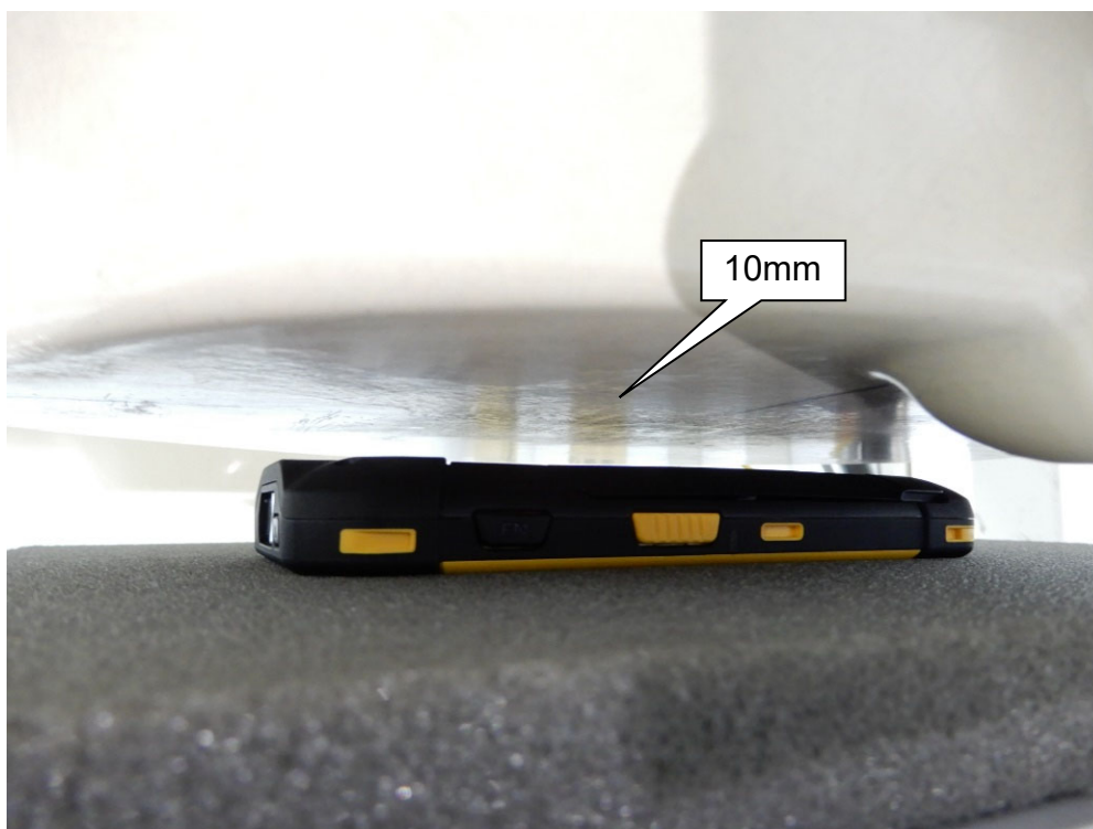
EUT Back_10mm
