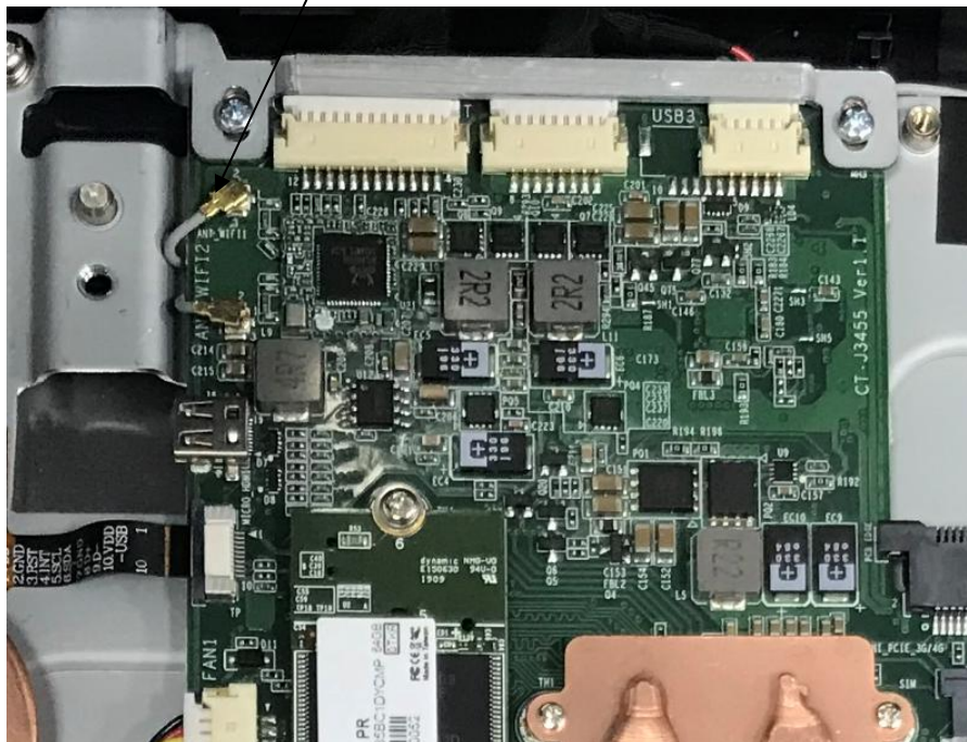
Bluetooth and WIFI Antenna
