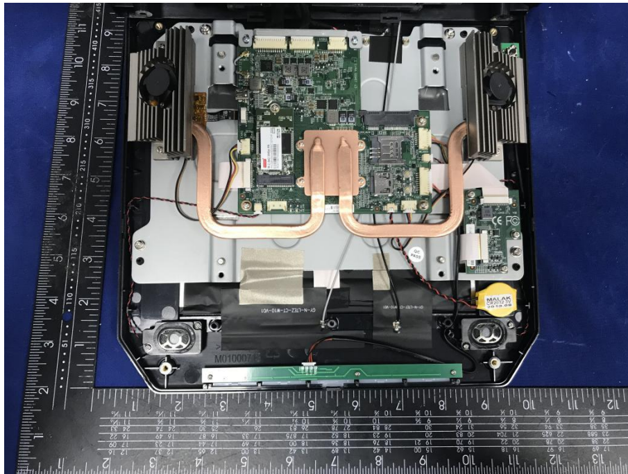
J3455 PCB
