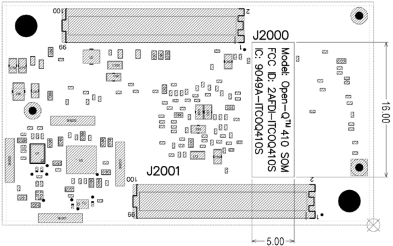
Bottom Side Drawing of Module with Dimensions (mm).
