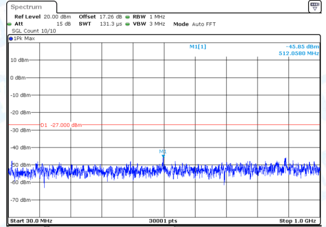
11AC80MIMO-Ant2-5610-30~1000-PASS
