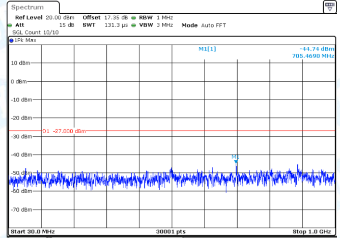
11AC40MIMO-Ant2-5710-30~1000-PASS
