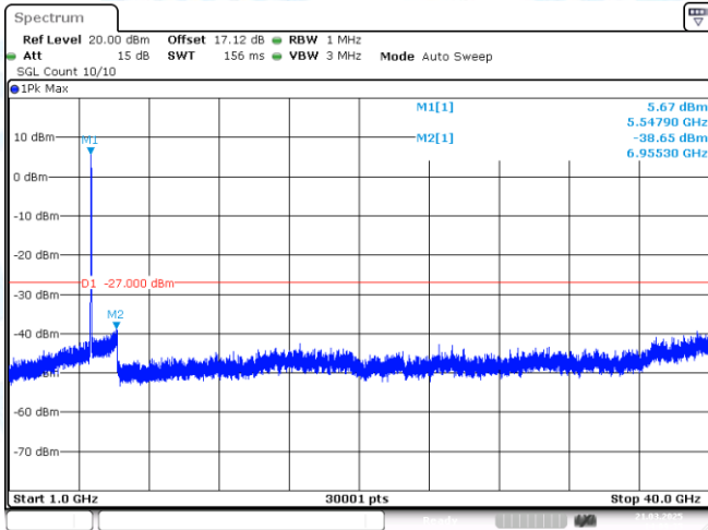
11AC40MIMO-Ant1-5550-1000~40000-PASS
