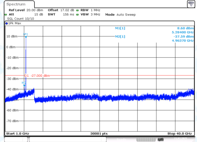
11AX20MIMO-Ant2-5280-1000~40000-PASS
