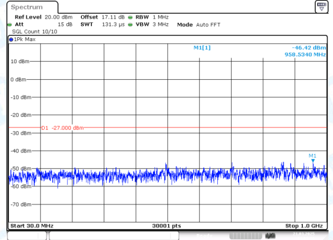
11AC40MIMO-Ant2-5510-30~1000-PASS
