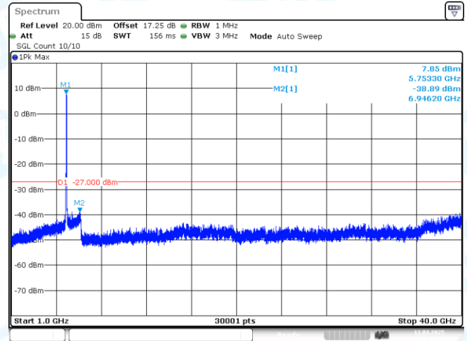
11AC40MIMO-Ant2-5755-1000~40000-PASS
