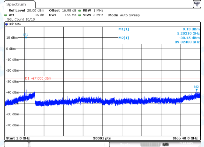
11AX20MIMO-Ant2-5200-1000~40000-PASS
