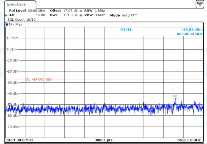
11AC40MIMO-Ant2-5230-30~1000-PASS
