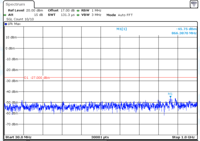
11AX20MIMO-Ant2-5180-30~1000-PASS
