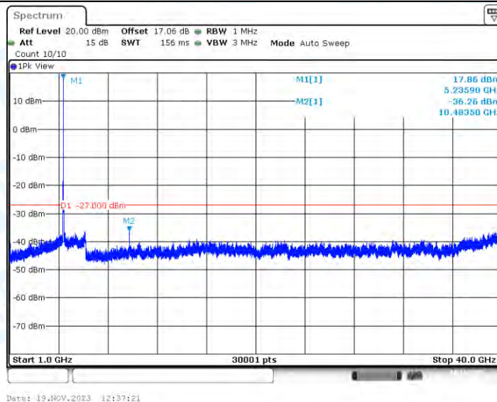
11AX20-CDD_Ant3_5240_30~1000
