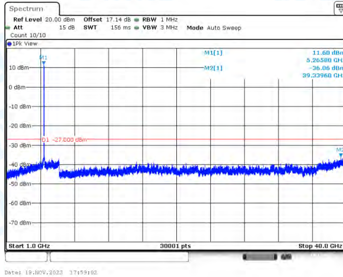
11AX40-CDD_Ant4_5270_30~1000
