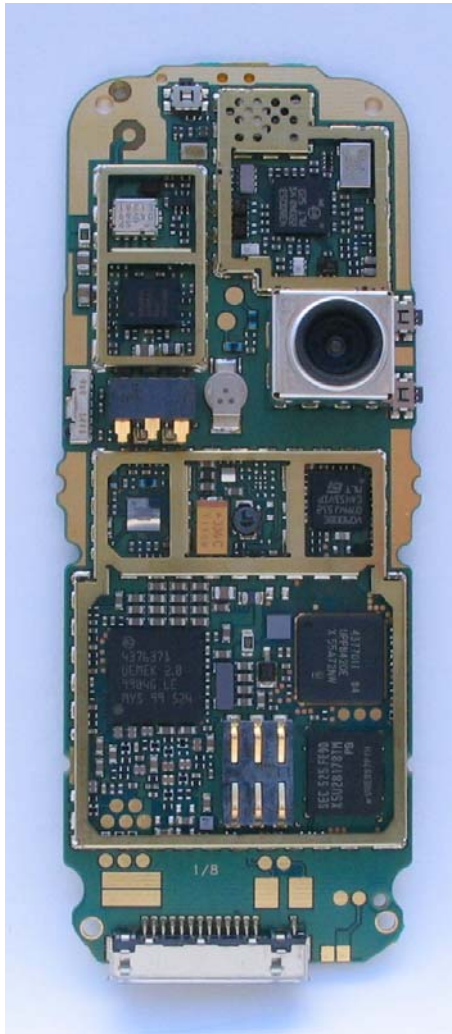
Shielding disassembled
