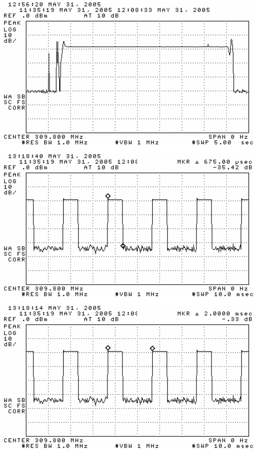
Figure 6.1(a). Transmissions modulation characteristics: (top) full transmission, (middle) pulse width, (bottom) pulse period. (310 MHz, 30% duty factor).
