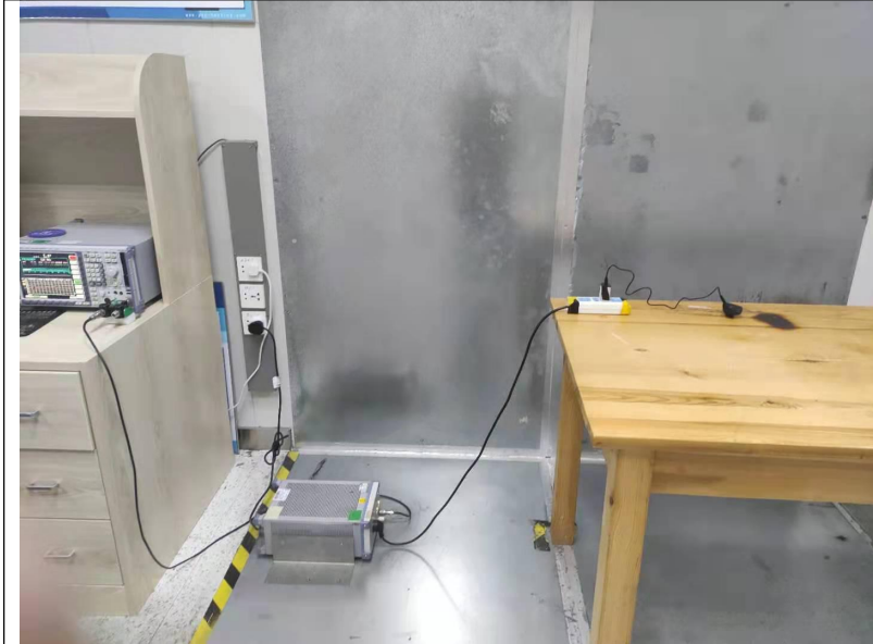
Radiated Spurious Emissions From 30MHz-1000MHz
