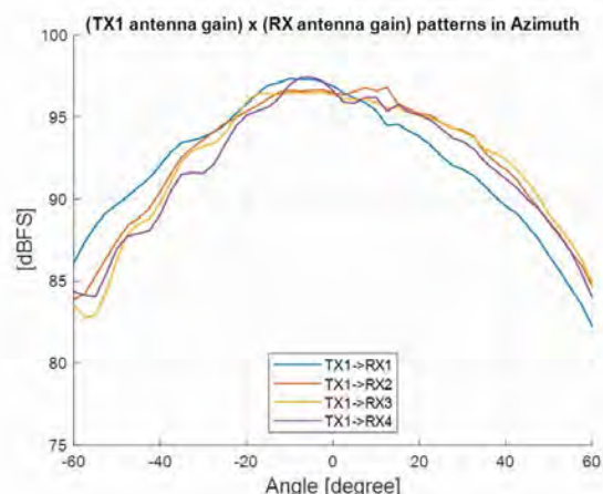
Figure 6-8. TX1 Antenna Radiation Pattern in Azimuth
