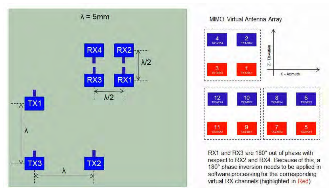
Figure 5-8. IWR6843AOP antenna placement MIMO array
