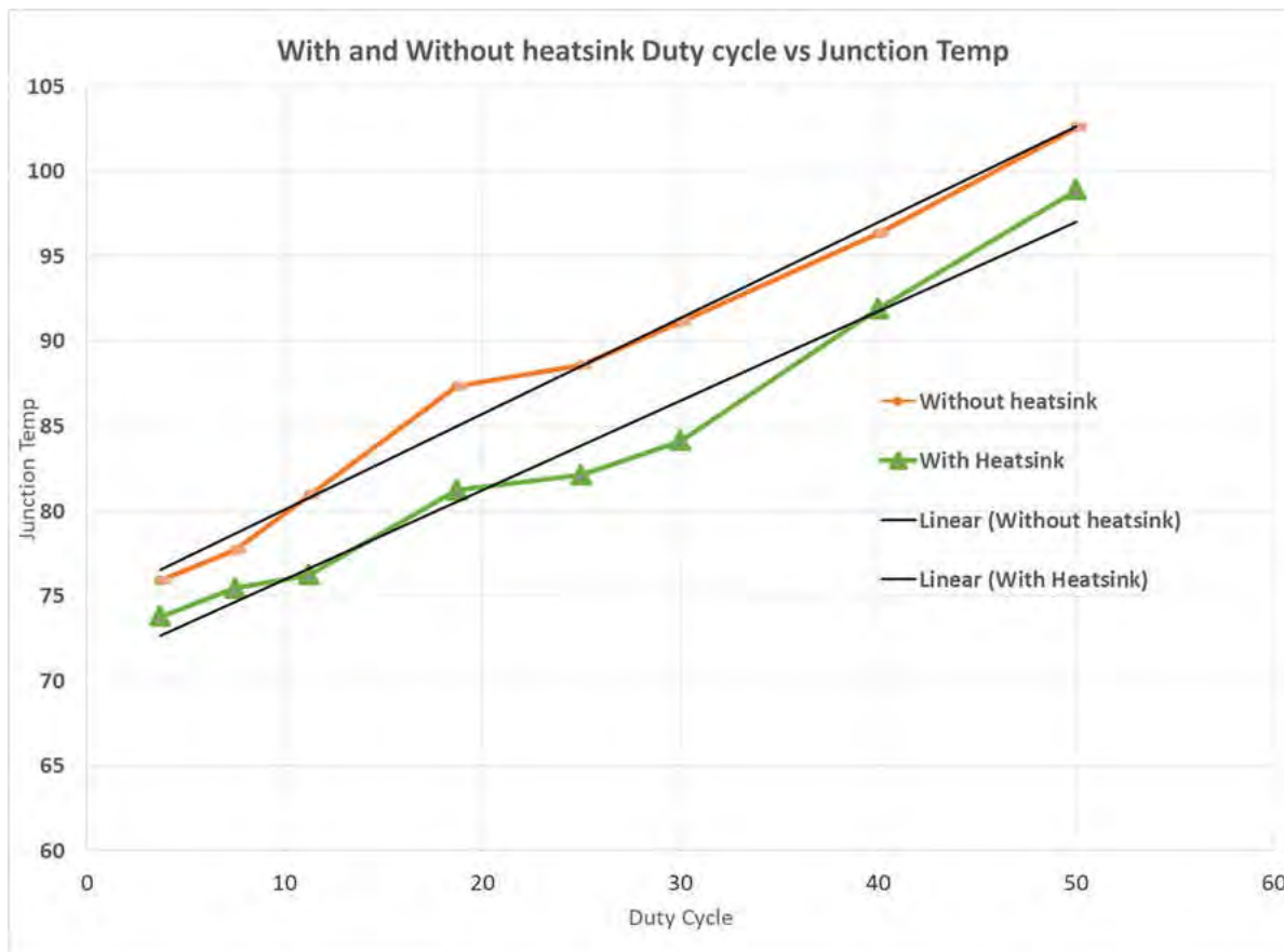
Figure 5-4. Duty Cycle versus Junction Temperature
