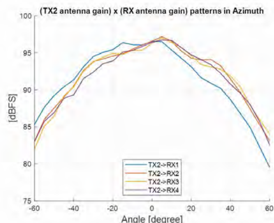
Figure 6-9. TX2 Antenna Radiation Pattern in Azimuth
