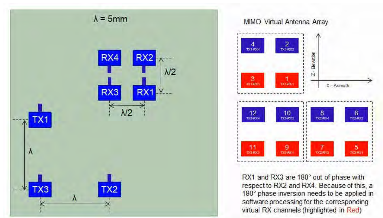
Figure 4-8. IWR6843AOP antenna placement MIMO array
