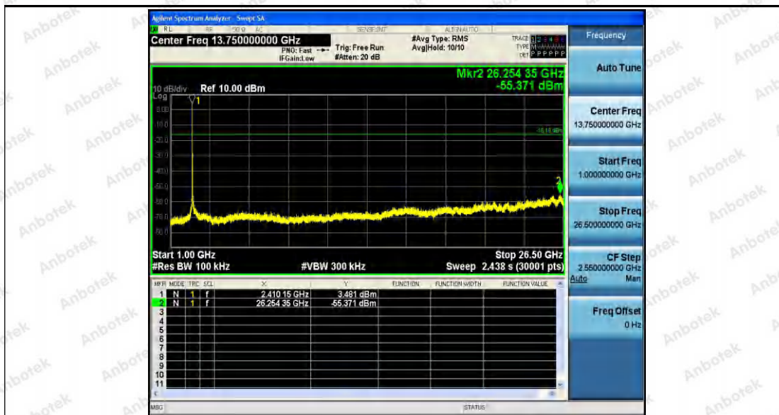
11B_Ant2_2412_0~Reference
