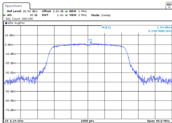
ac20_5240MHz_Chain 0
