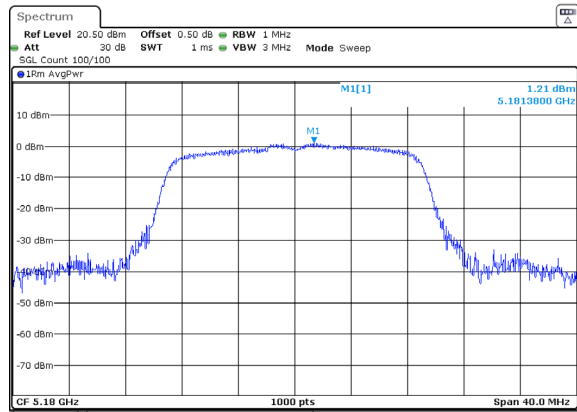
ac20_5180MHz_Chain 0
