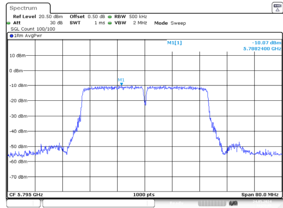
ac40_5795MHz_Chain 0
