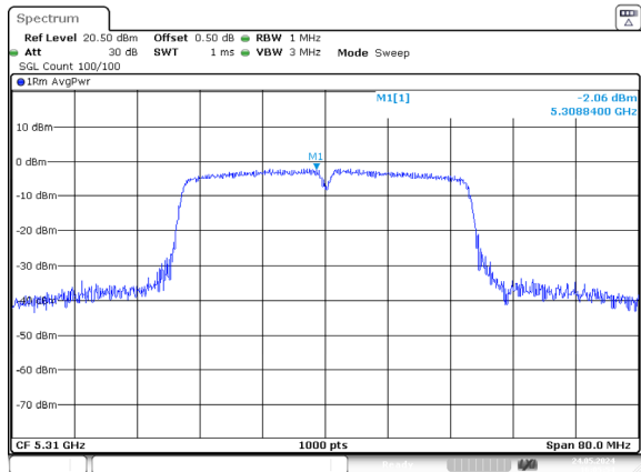
ac40_5310MHz_Chain 0
