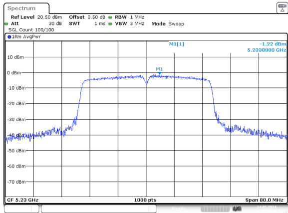
ac40_5230MHz_Chain 0
