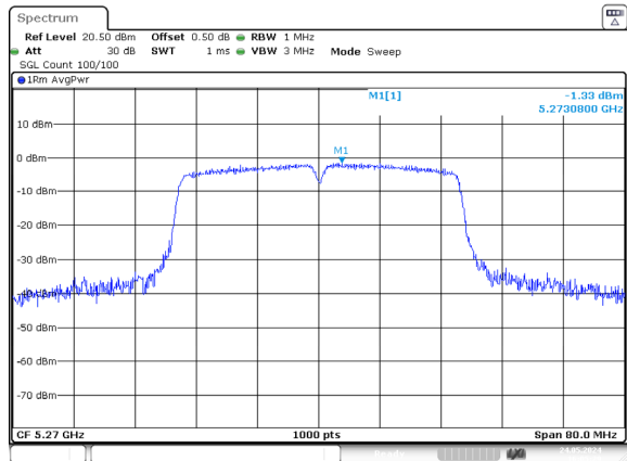
ac40_5270MHz_Chain 0
