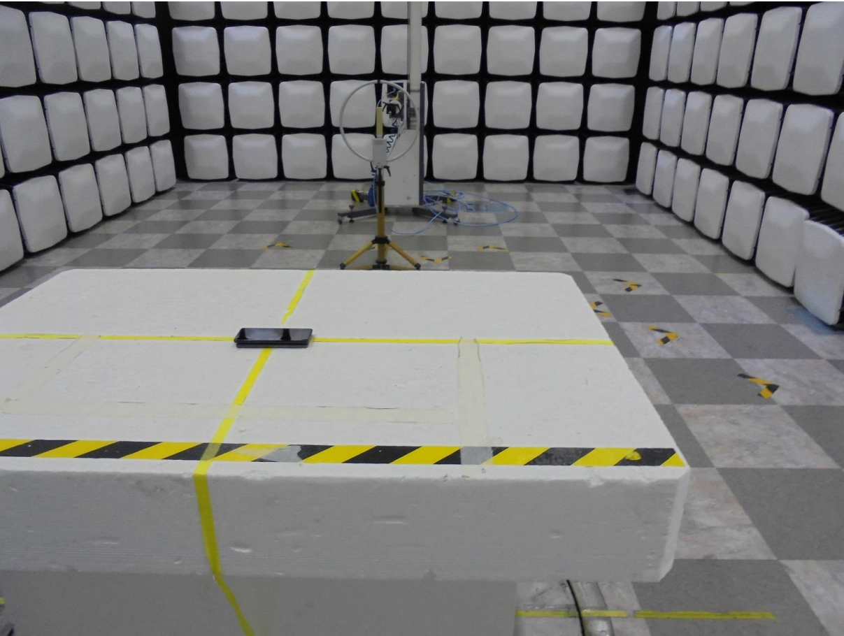
WPT Radiated Test Setup Photo for below 30 MHz: Phone to Clock(Position: Alignment)
