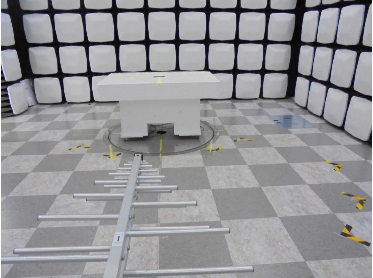
NFC Radiated Test Setup Photo for 30 MHz ~ 1 GHz :
