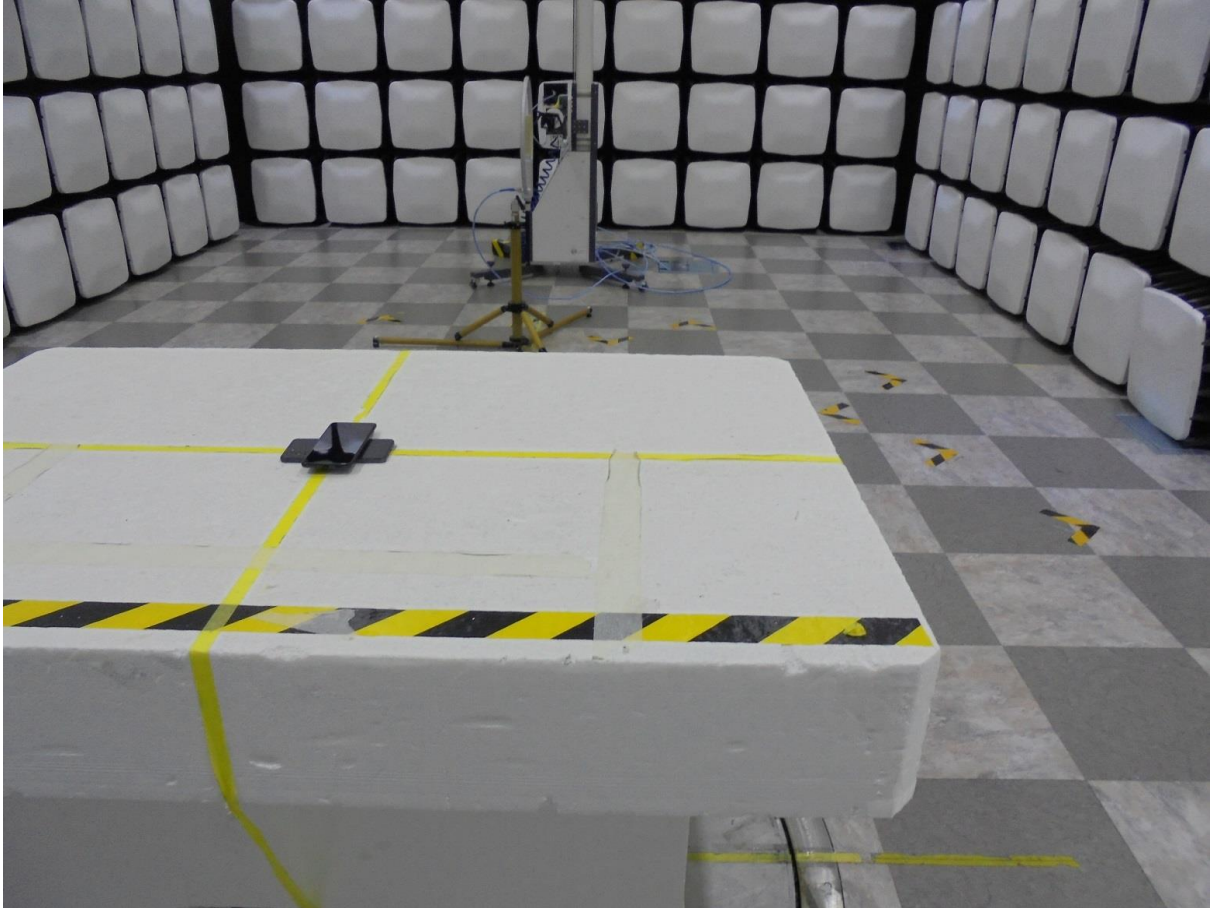
Phone to Clock(Position: Cross)
