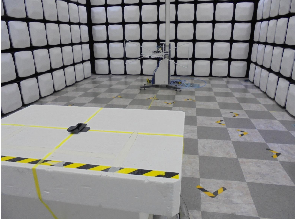
Phone to Phone(Position: Cross)
