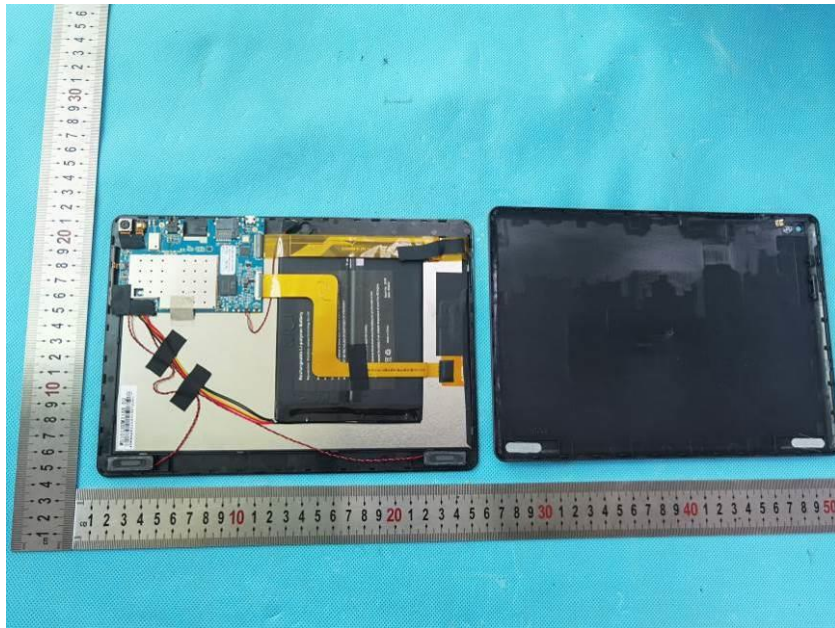
WIFI/BT ANT
