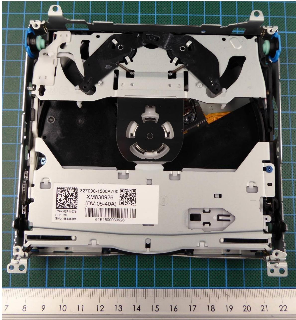
160090_28. jpg: EUT – Main Unit – CD drive without PCB top view
