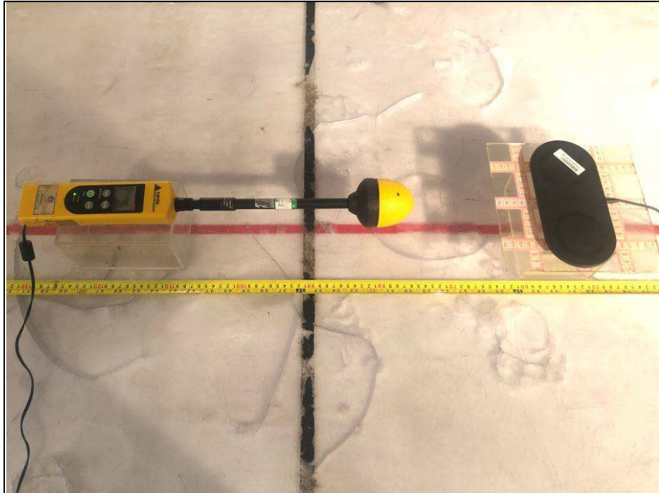
Electric Field
