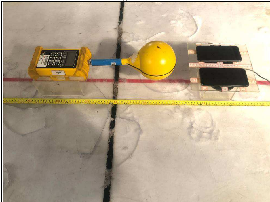
Magnetic Field
