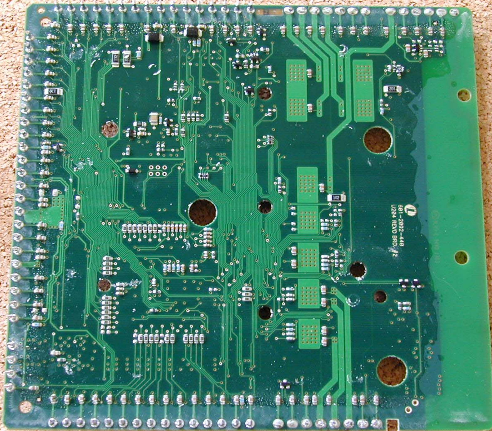
PCB 2 (bottom)
