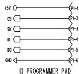
ID PROGRAMMER PAD
