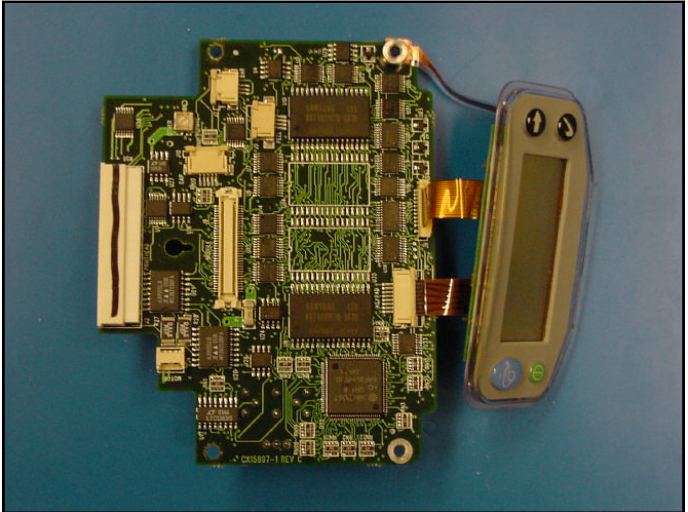
PHOTOGRAPH 18: PCB1 TOP WITH LCD DISPLAY
