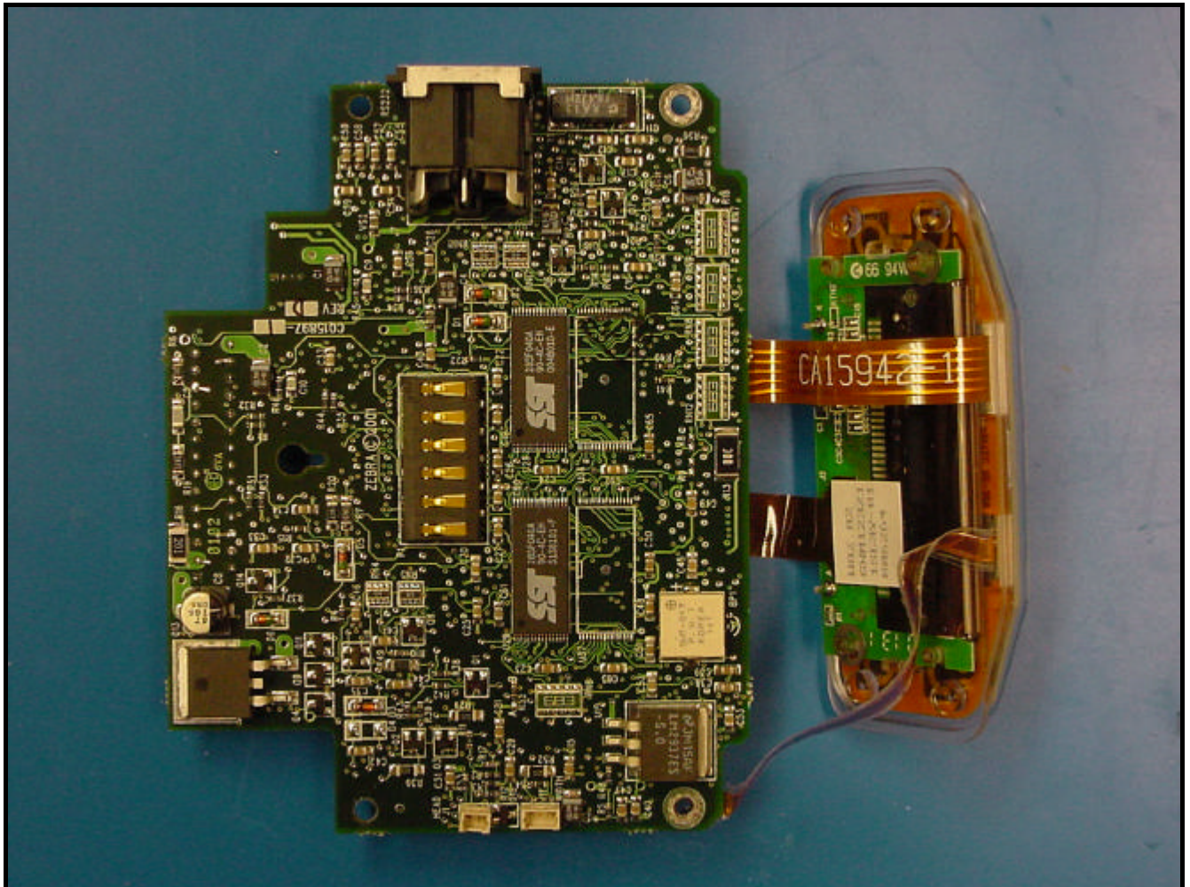
PHOTOGRAPH 20: PCB1 BOTTOM WITH LCD DISPLAY
