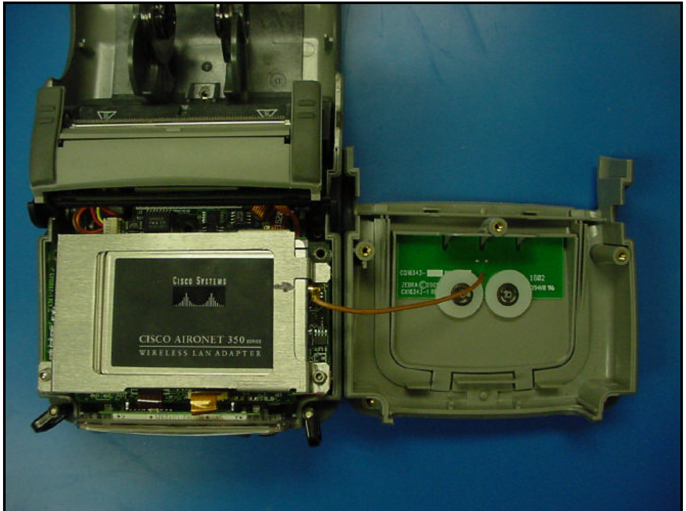
PHOTOGRAPH 25: WLAN CONNECTION TO ANTENNA
