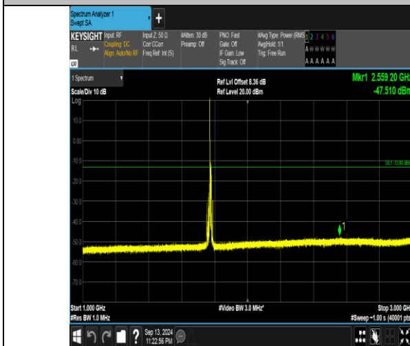
Band66_10MHz_16QAM_132622_1RB#0_1000~3000_1000~3000
