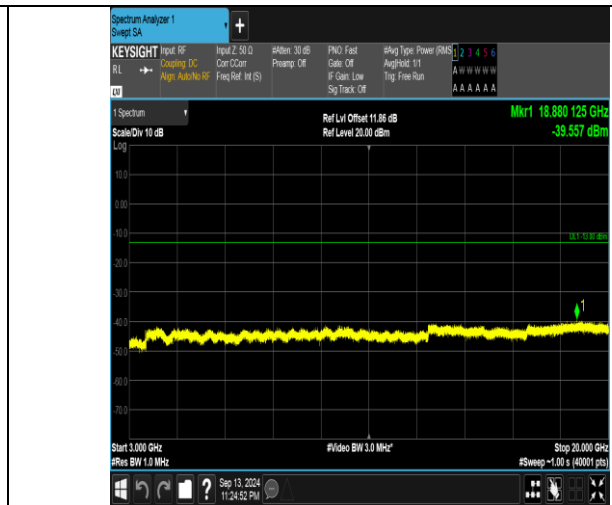
Band66_10MHz_16QAM_132622_1RB#49_3000~20000_3000~20000
