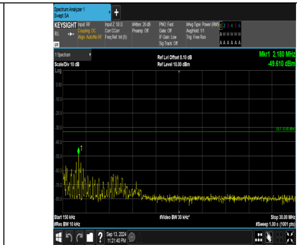
Band66_10MHz_QPSK_132622_1RB#0_0.15~30_0.15~30
