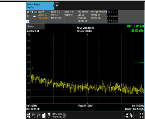
Band66_10MHz_16QAM_132622_1RB#0_0.009~0.15_0.009~0.15
