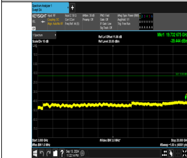
Band66_10MHz_QPSK_132622_1RB#0_3000~20000_3000~20000
