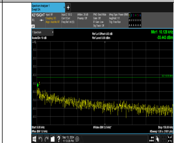
Band66_10MHz_16QAM_132022_1RB#49_0.009~0.15_0.009~0.15
