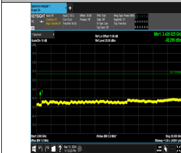
Band66_10MHz_QPSK_132022_1RB#49_3000~20000_3000~20000
