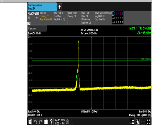
Band66_10MHz_QPSK_132622_50RB#0_1000~3000_1000~3000
