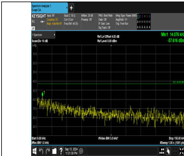
Band66_10MHz_QPSK_132622_1RB#0_0.009~0.15_0.009~0.15
