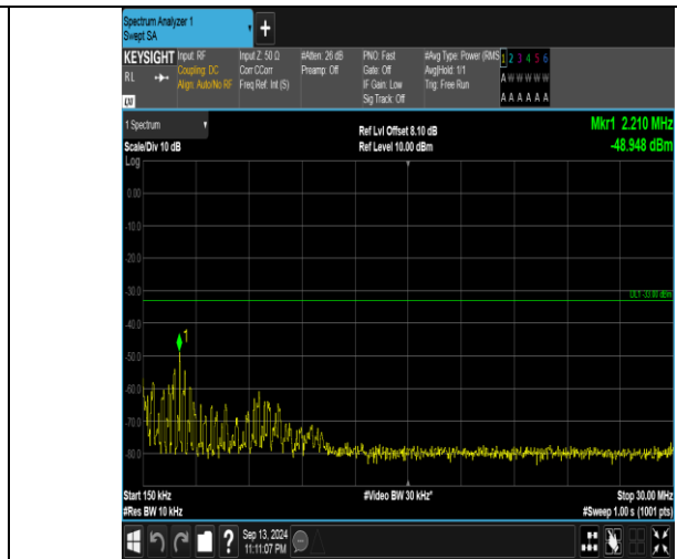
Band66_10MHz_QPSK_132022_1RB#0_0.15~30_0.15~30
