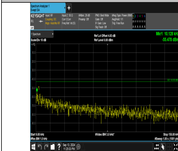
Band66_10MHz_QPSK_132622_50RB#0_0.009~0.15_0.009~0.15
