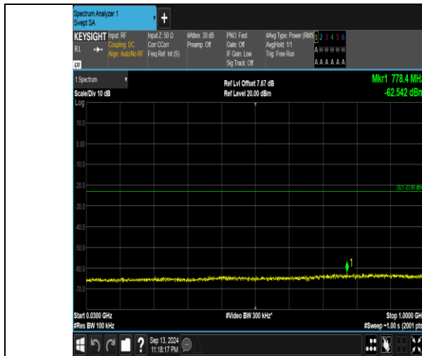
Band66_10MHz_QPSK_132322_1RB#49_30~1000_30~1000
