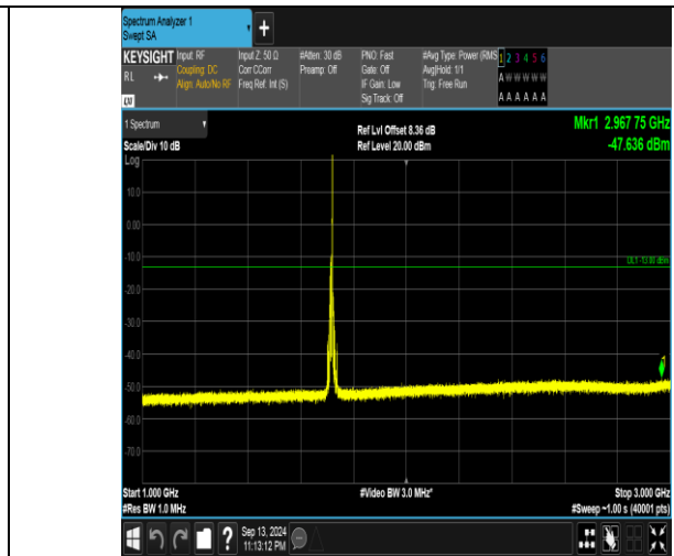
Band66_10MHz_QPSK_132022_1RB#49_1000~3000_1000~3000
