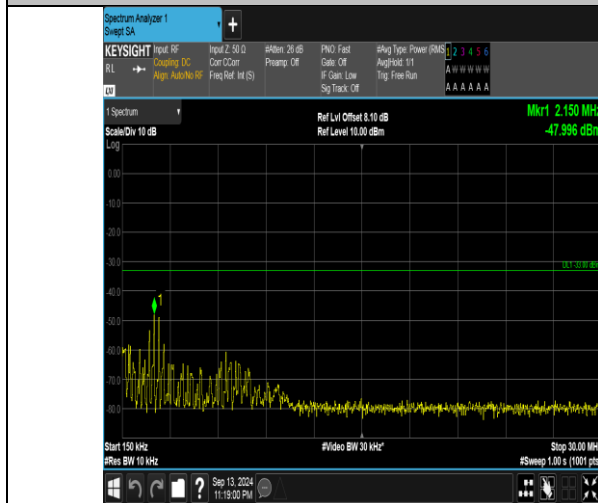
Band66_10MHz_16QAM_132322_1RB#49_0.15~30_0.15~30
