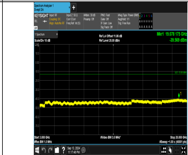
Band66_10MHz_16QAM_132322_1RB#0_3000~20000_3000~20000
