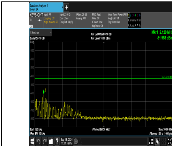
Band66_10MHz_16QAM_132322_1RB#0_0.15~30_0.15~30
