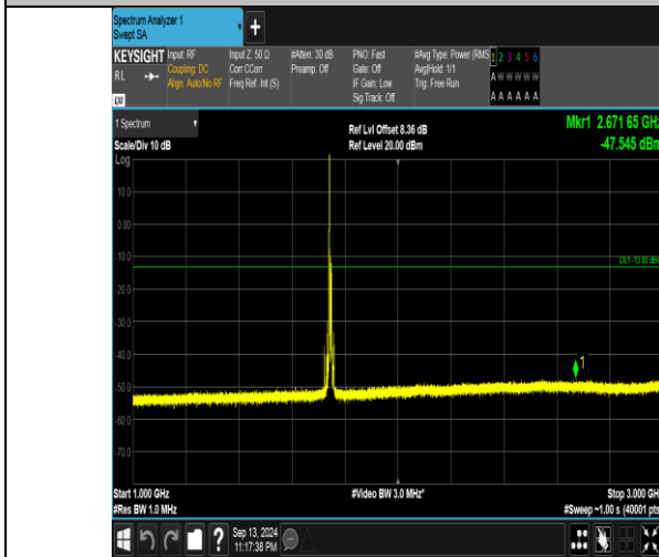
Band66_10MHz_16QAM_132322_1RB#0_1000~3000_1000~3000
