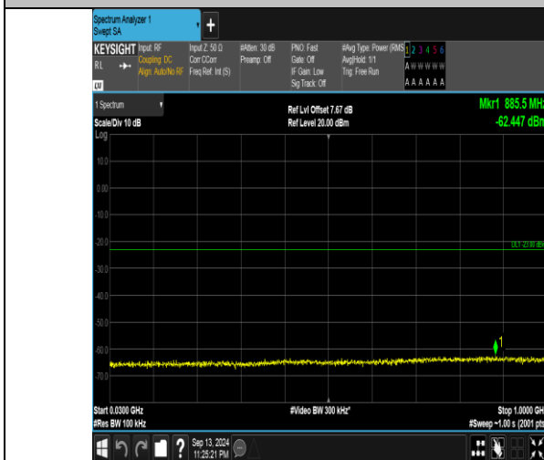
Band66_10MHz_QPSK_132622_50RB#0_30~1000_30~1000
