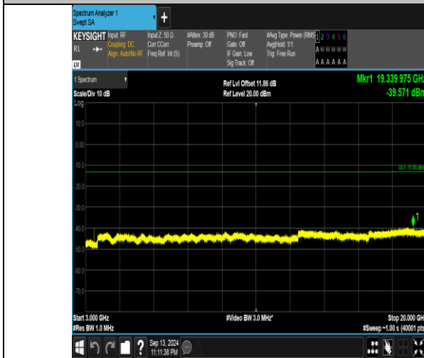
Band66_10MHz_QPSK_132022_1RB#0_3000~20000_3000~20000
