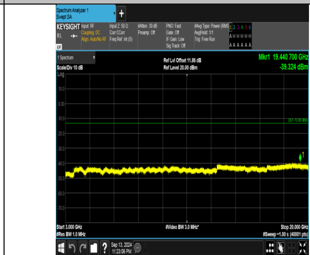
Band66_10MHz_16QAM_132622_1RB#0_3000~20000_3000~20000
