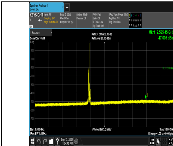
Band66_10MHz_16QAM_132622_1RB#49_1000~3000_1000~3000
