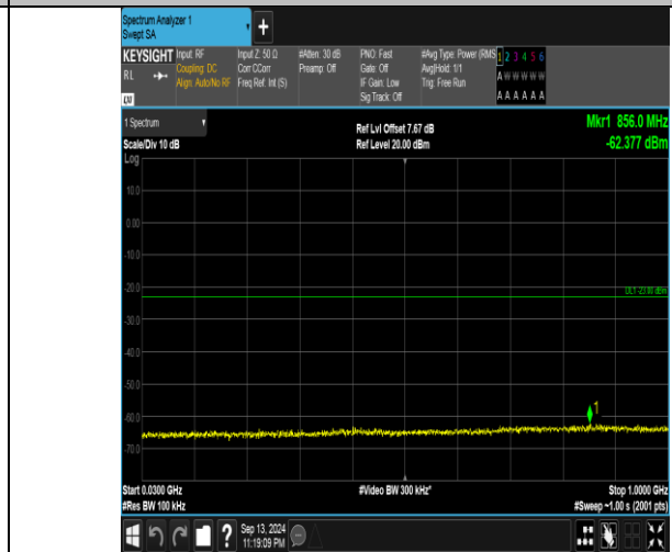
Band66_10MHz_16QAM_132322_1RB#49_30~1000_30~1000
