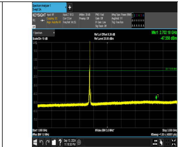
Band66_10MHz_QPSK_132322_1RB#49_1000~3000_1000~3000
