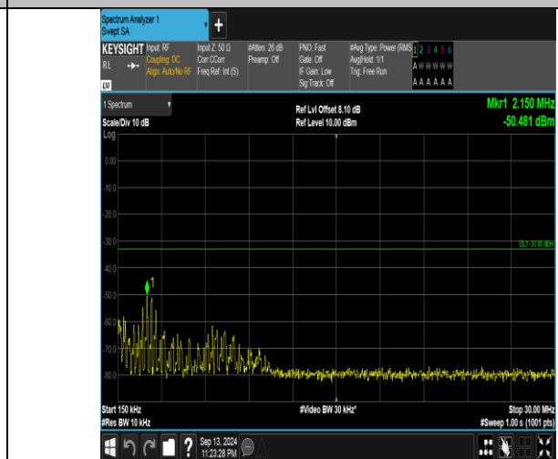
Band66_10MHz_QPSK_132622_1RB#49_0.15~30_0.15~30
