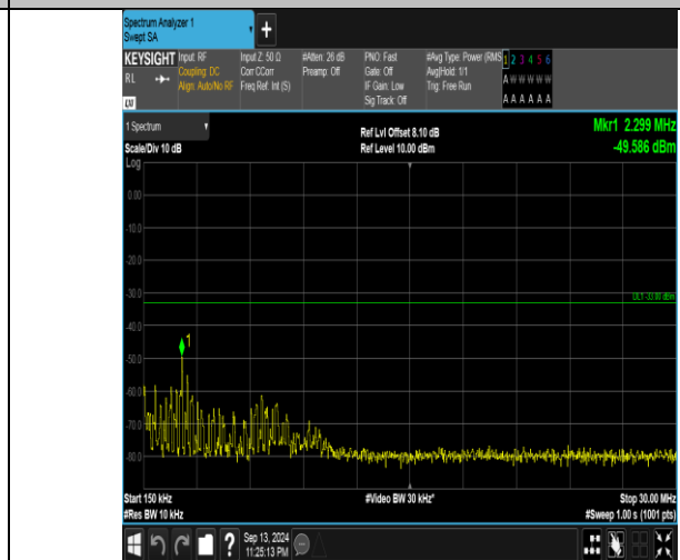
Band66_10MHz_QPSK_132622_50RB#0_0.15~30_0.15~30
