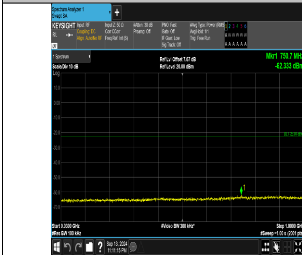
Band66_10MHz_QPSK_132022_1RB#0_30~1000_30~1000
