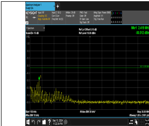
Band66_10MHz_16QAM_132622_1RB#0_0.15~30_0.15~30
