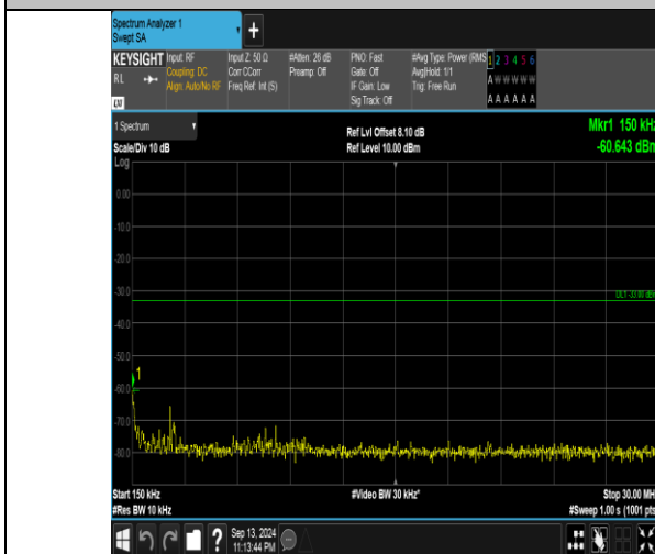
Band66_10MHz_16QAM_132022_1RB#49_0.15~30_0.15~30
