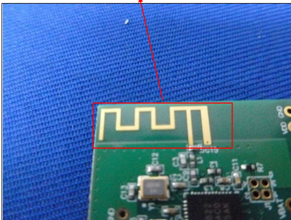
BT_LE Antenna
