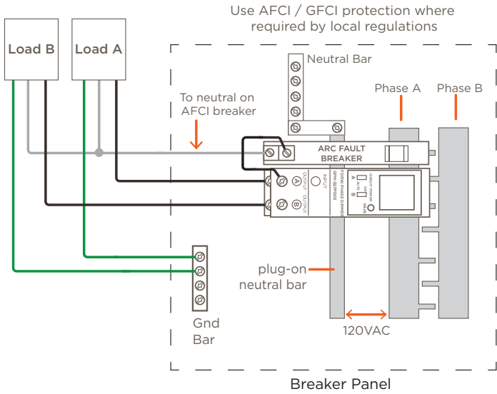
Plug-on Neutral Bus Bar with ARC Fault Breakers
