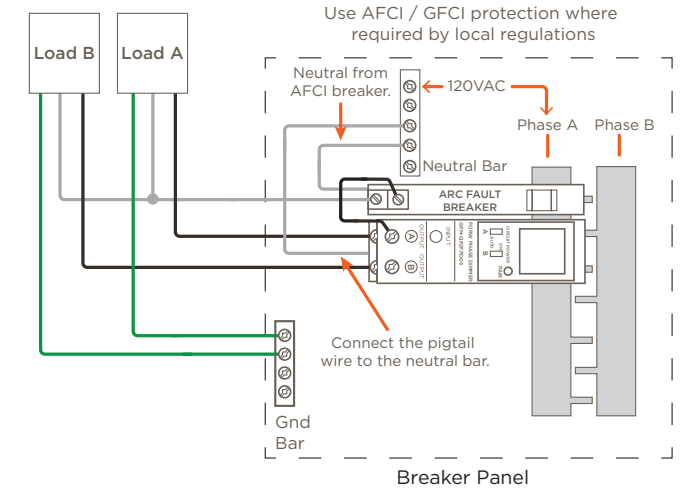
Standard Neutral Bus Bar with ARC Fault Breakers
