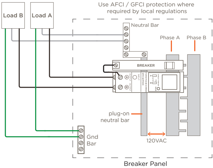
Plug-on Neutral Bus Bar with Standard Breakers
