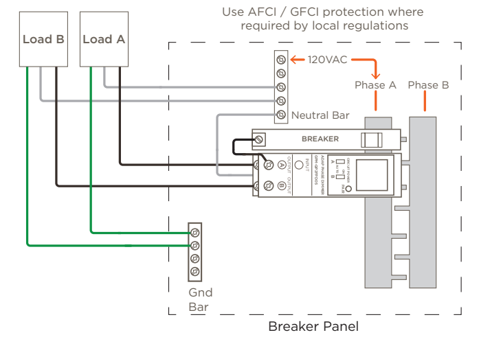
Standard Neutral Bus Bar with Standard Breakers
