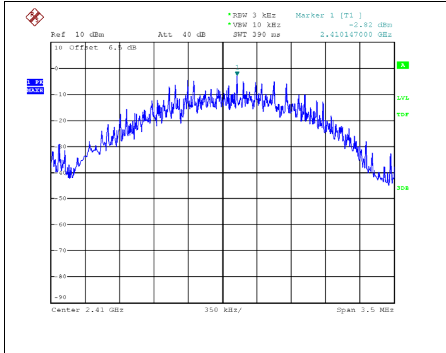
MESH _ Middle frequency Peak Power Spectral Density
