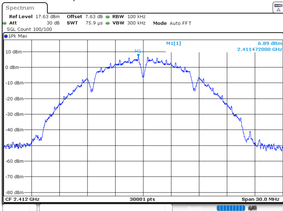
Tx. Spurious NVNT 802.11b 2412MHz Ant 0 Ref
