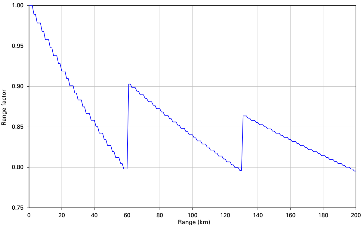
Figure 76 Range adjustment for PTP 700, symmetry 1:1, optimization TDM, bandwidth 15 MHz
