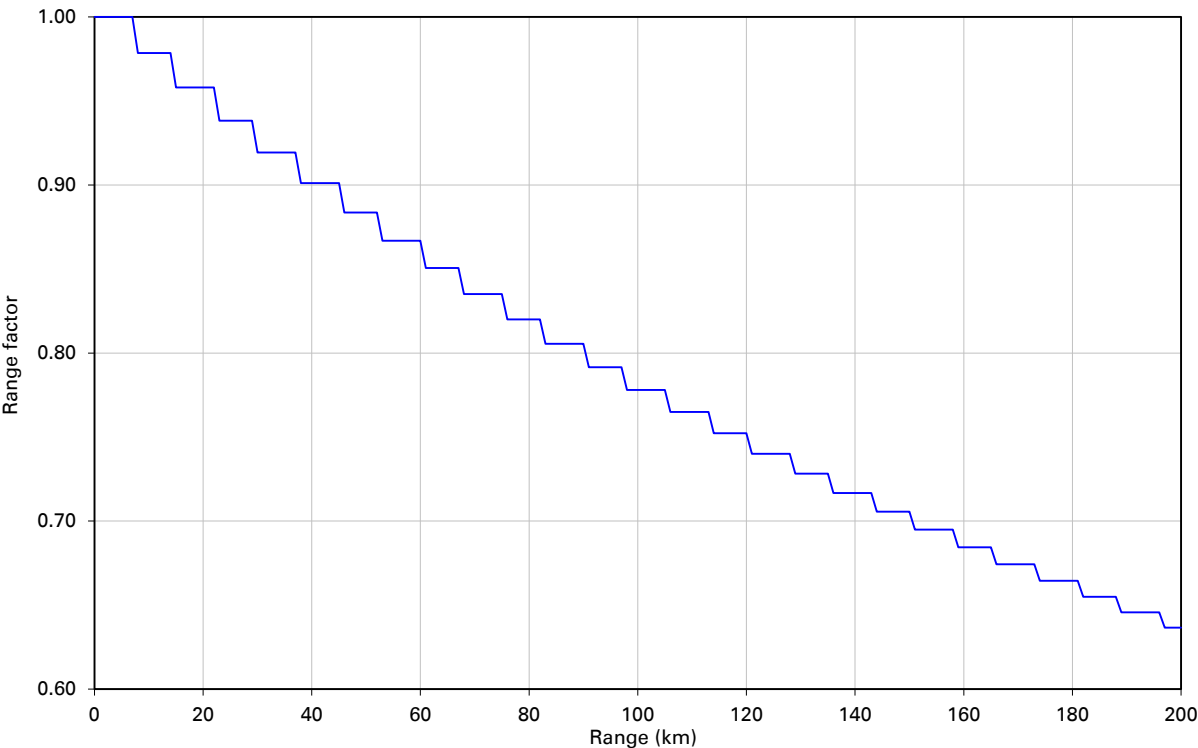
Figure 72 Range adjustment for PTP 700, symmetry 1:1, optimization TDM, bandwidth 45 MHz
