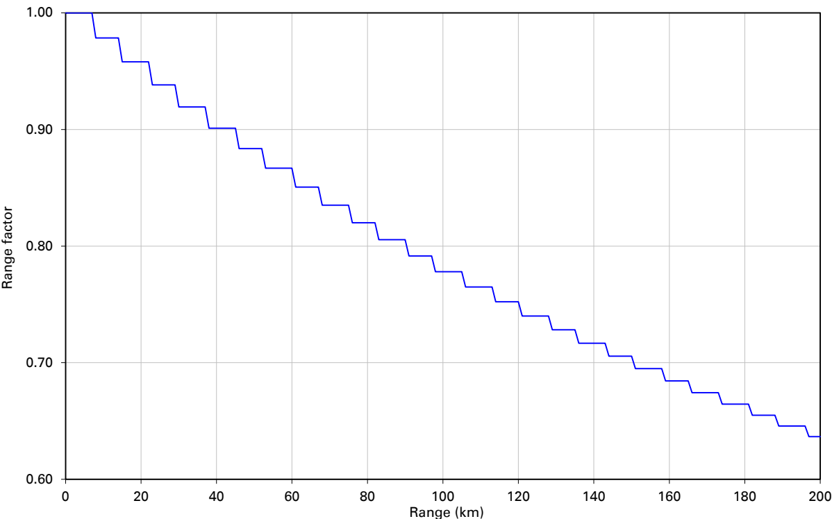
Figure 78 Range adjustment for PTP 700, symmetry 1:1, optimization TDM, bandwidth 5 MHz
