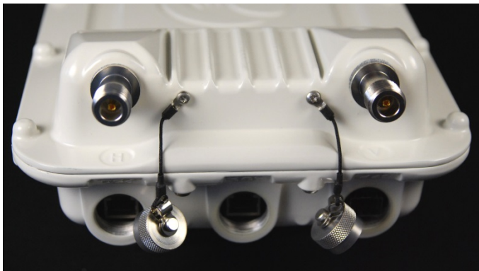
Figure 16 Connectorized ODU antenna interfaces
