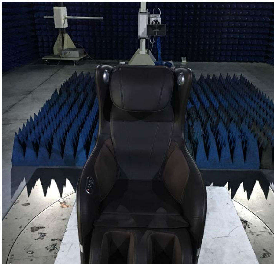
Photograph of set-up for Radiated Emission above 1GHz
