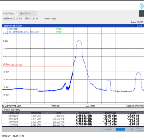
1-N77-3700-3980--30-10-L-1-DFT-PI2BPSK-Edge_1R B_Left-1@0-Ant0-PASS-see graph
