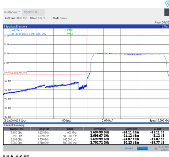
1-N77-3700-3980--30-10-L-6-CP-QPSK-Outer_Ful l-24@0-Ant0-PASS-see graph
