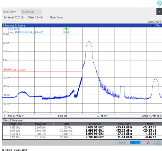
1-N77-3700-3980--30-10-L-4-CP-QPSK-Edge_1RB_L eft-1@0-Ant0-PASS-see graph
