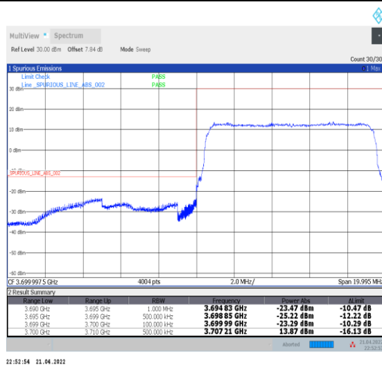
1-N77-3700-3980--30-10-L-3-DFT-PI2BPSK-Outer _Full-24@0-Ant0-PASS-see graph
