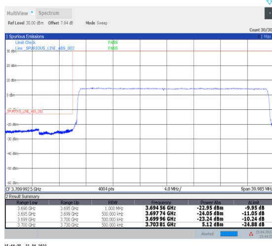
1-N77-3700-3980--30-30-L-6-CP-QPSK-Outer_Ful l-78@0-Ant0-PASS-see graph
