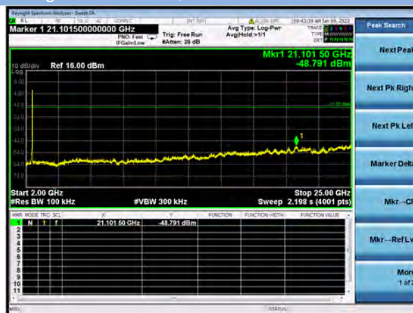
802.11g CHANNEL 11, SPURIOUS 2 GHz ~ 25 GHz
