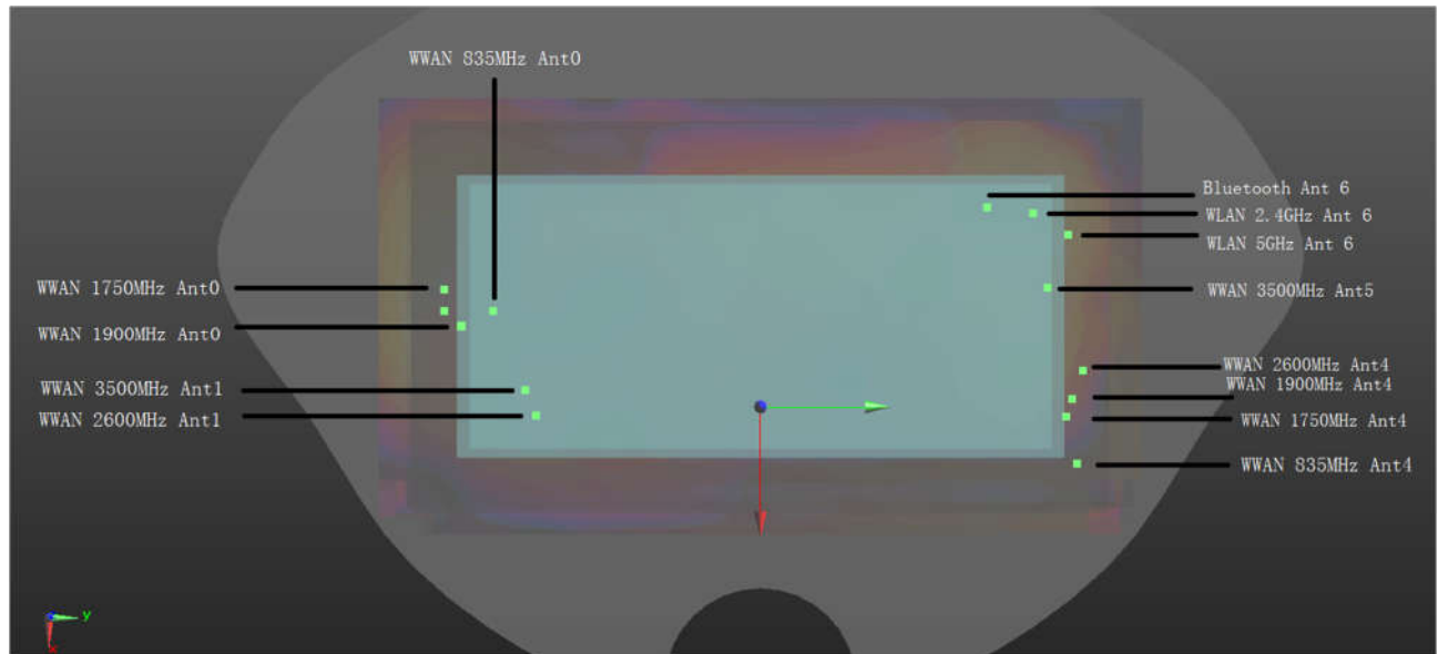
WWAN+2.4GHz/WWAN+5GHz+Bluetooth (5mm)_Back for Hotspot
