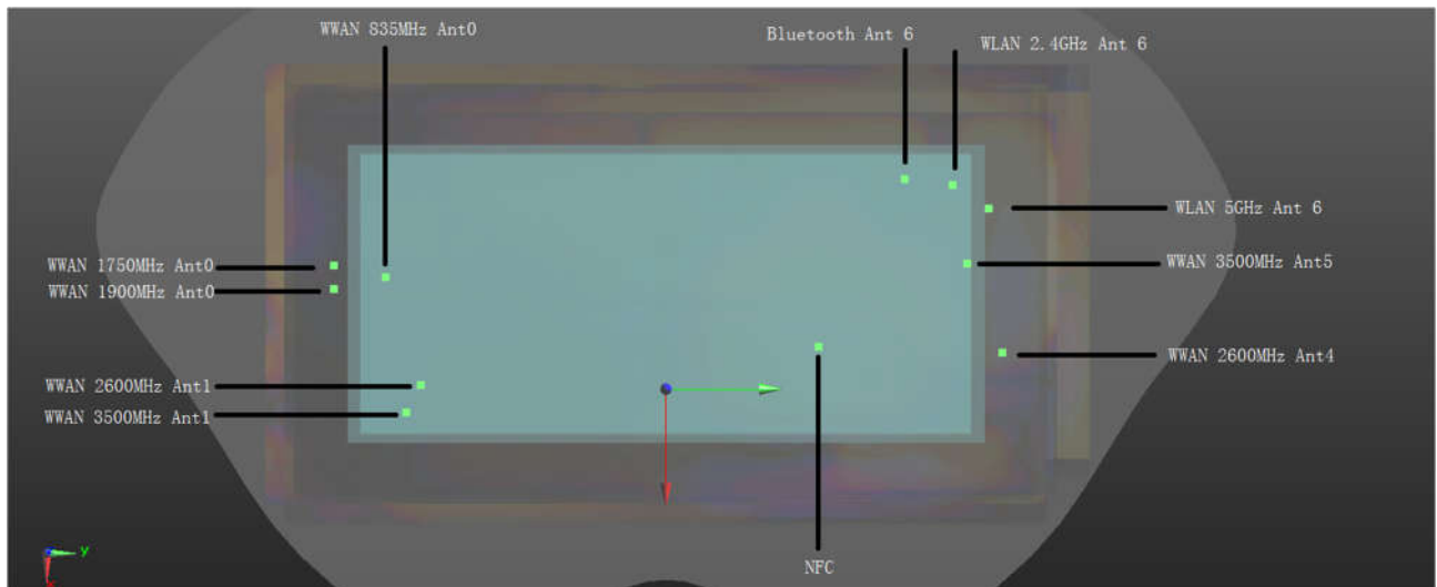
WWAN+2.4GHz+NFC/WWAN+5GHz+Bluetooth+NFC(0mm)_Back
