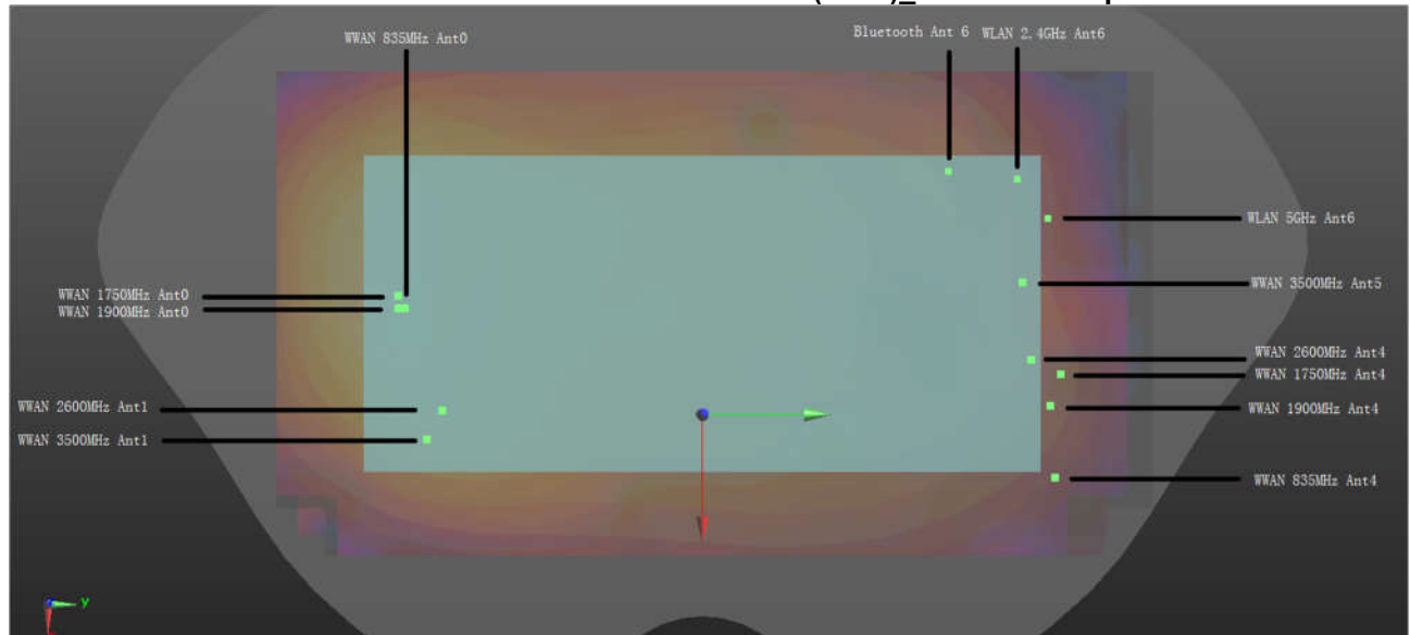
WWAN+2.4GHz/WWAN+5GHz+Bluetooth (5mm)_Back for Body-worn
