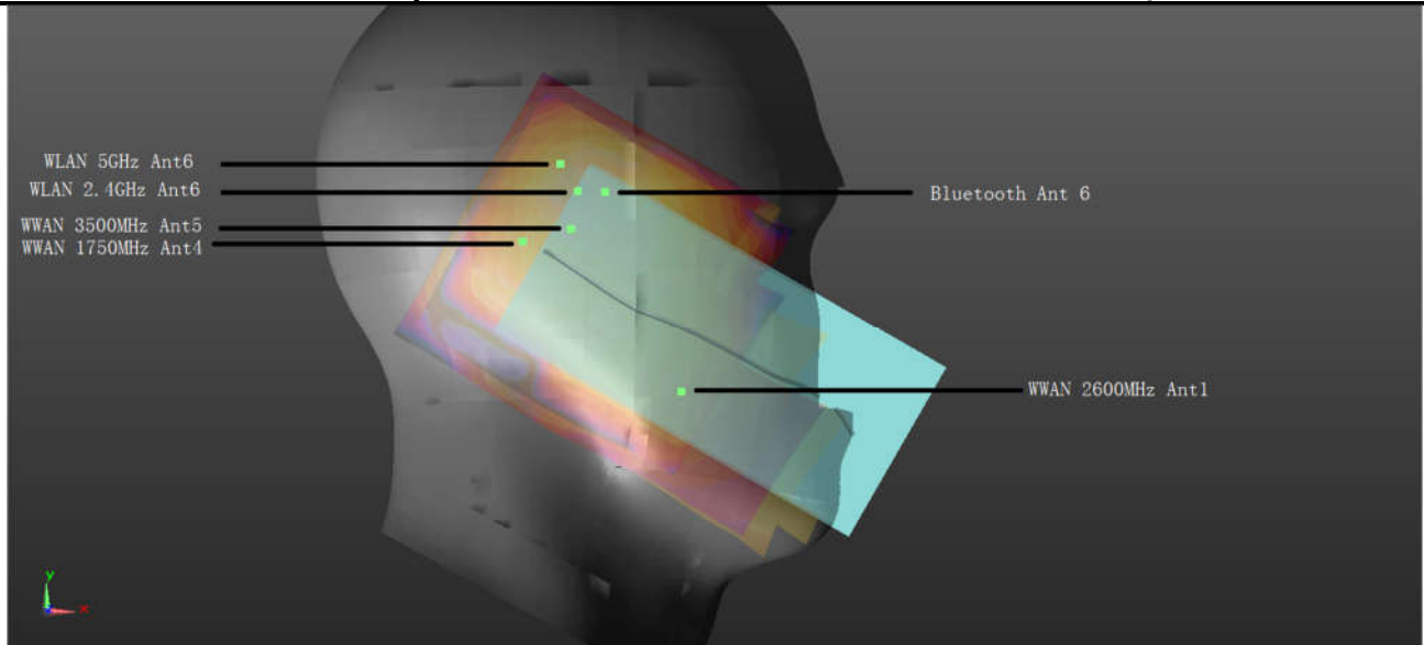
WWAN+2.4GHz/WWAN+5GHz+Bluetooth(0mm)_Left Check
