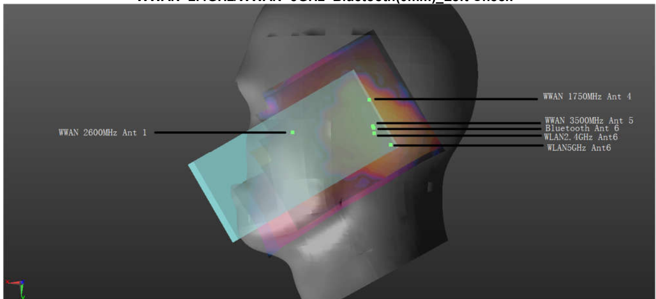
WWAN+2.4GHz/WWAN+5GHz+Bluetooth (0mm)_Right Tilted
