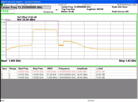
Band 25 5MHz/1912.5/High 16QAM 1@0
