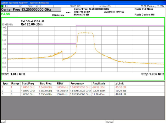
Band 25 1.4MHz/1850.7/Low 16QAM 6@0
