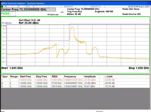
Band 25 1.4MHz/1850.7/Low 16QAM 1@0
