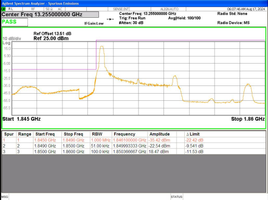
Band 25 5MHz/1852.5/Low 16QAM 1@0
