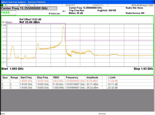
Band 25 5MHz/1912.5/High QPSK 1@24
