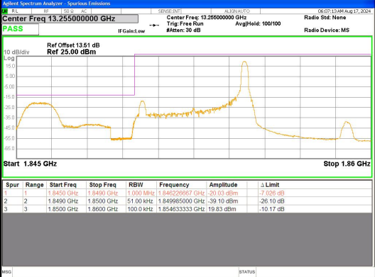
Band 25 5MHz/1852.5/Low QPSK 1@24
