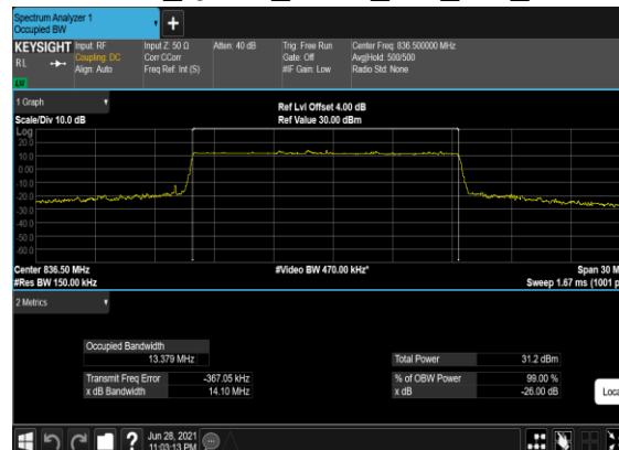
N5(15M)_DFT-s- OFDM_QPSK_Outer_Full_Mid_CH
