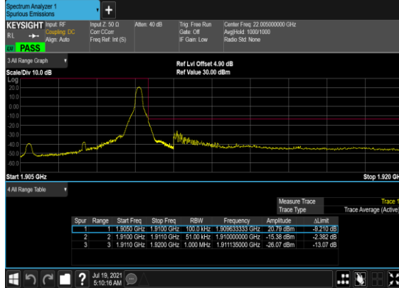
B5_N2(5M)_DFT-s- OFDM_QPSK_Edge_1RB_Right_High_CH
