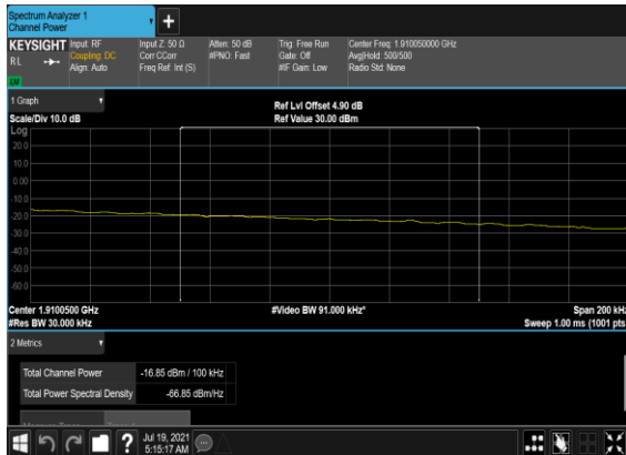
B5_N2(10M)_DFT-s- OFDM_QPSK_Edge_1RB_Right_High_CH
