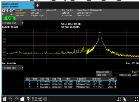
B5_N2(20M)_DFT-s- OFDM_QPSK_Edge_1RB_Left_Low_CH
