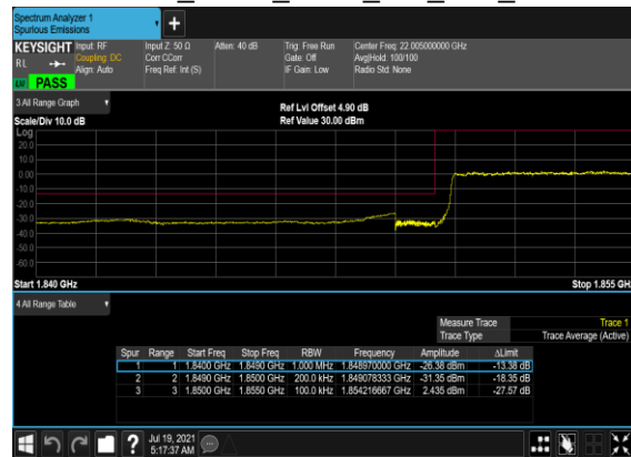
B5_N2(20M)_DFT-s- OFDM_BPSK_Outer_Full_Low_CH
