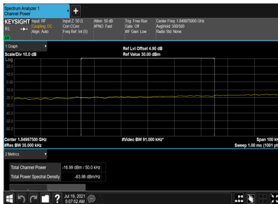
B5_N2(5M)_DFT-s- OFDM_QPSK_Edge_1RB_Left_Low_CH_CHP PASS
