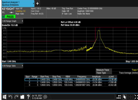
B5_N2(10M)_DFT-s- OFDM_QPSK_Edge_1RB_Left_Low_CH
