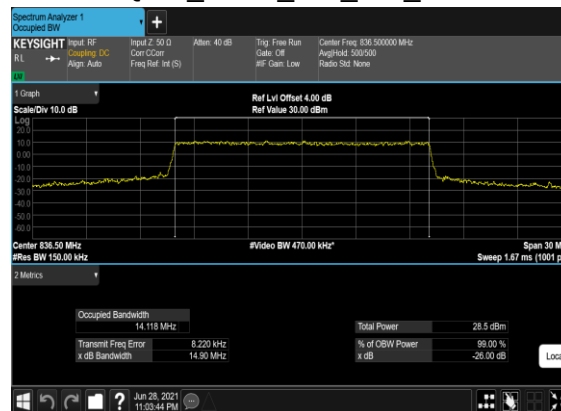
N5(15M)_CP-OFDM_16 QAM_Outer_Full_Mid_CH
