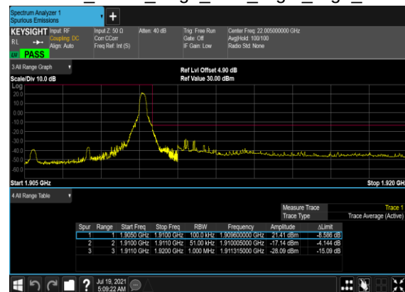
B5_N2(5M)_DFT-s- OFDM_BPSK_Edge_1RB_Right_High_CH
