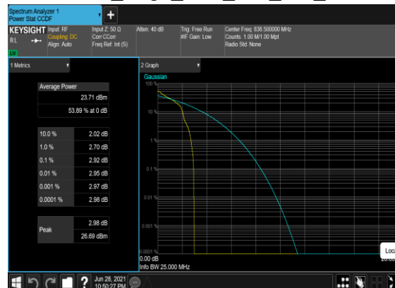
N5(20M)_DFT-s-OFDM_PI_2- BPSK_Edge_1RB_Left_Mid_CH
