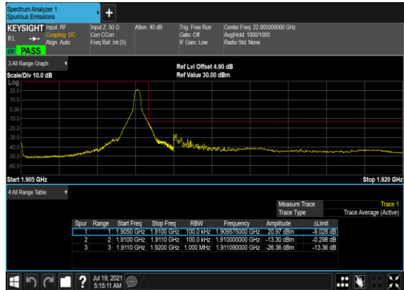
B5_N2(10M)_DFT-s- OFDM_QPSK_Edge_1RB_Right_High_CH
