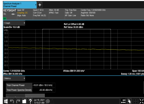
B5_N2(5M)_DFT-s- OFDM_QPSK_Edge_1RB_Right_High_CH_ch P_PASS
