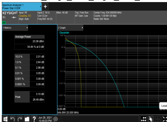
N5(20M)_DFT-s-OFDM_PI_2- BPSK_Edge_1RB_Right_Low_CH
