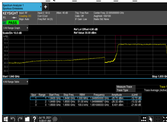
B5_N2(5M)_DFT-s- OFDM_QPSK_Outer_Full_Low_CH
