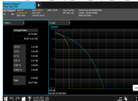
N5(20M)_DFT-s- OFDM_QPSK_Edge_1RB_Right_Mid_CH
