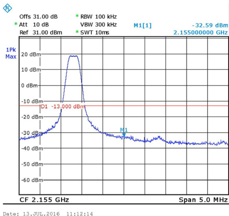
Figure 53. — GSM 2153.8 MHz
