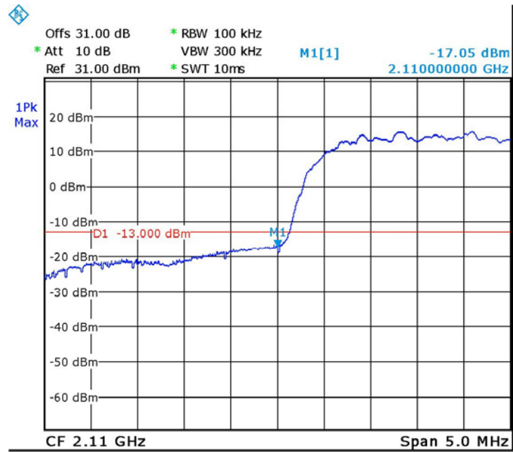
Figure 56. — W-CDMA 2112.5 MHz
