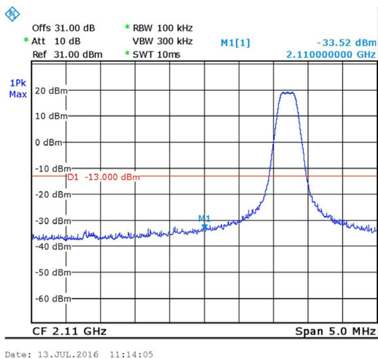
Figure 52. — GSM 2111.2 MHz
