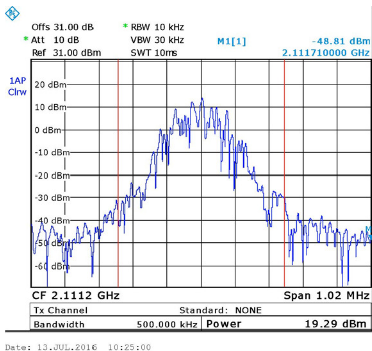
Figure 11. — GSM (2111.2 MHz)
