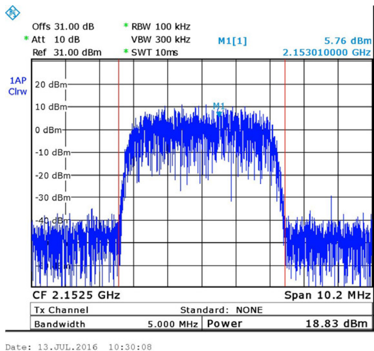
Figure 19. — W-CDMA (2152.5MHz)
