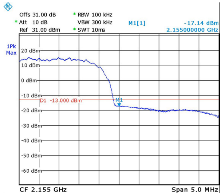
Figure 57. — W-CDMA 2152.5 MHz
