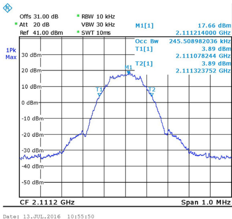
Figure 29. — GSM (2111.2 MHz) OUT
