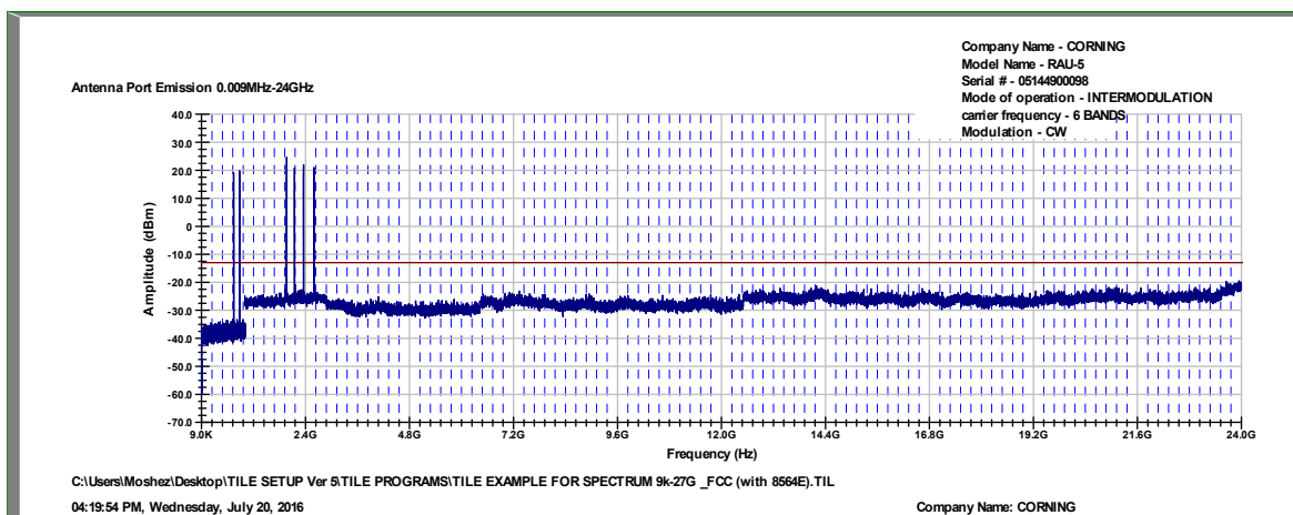
Figure 61 Intermodulation Conducted
