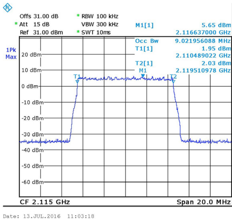
Figure 22. — LTE 64QAM (2115.0 MHz) IN
