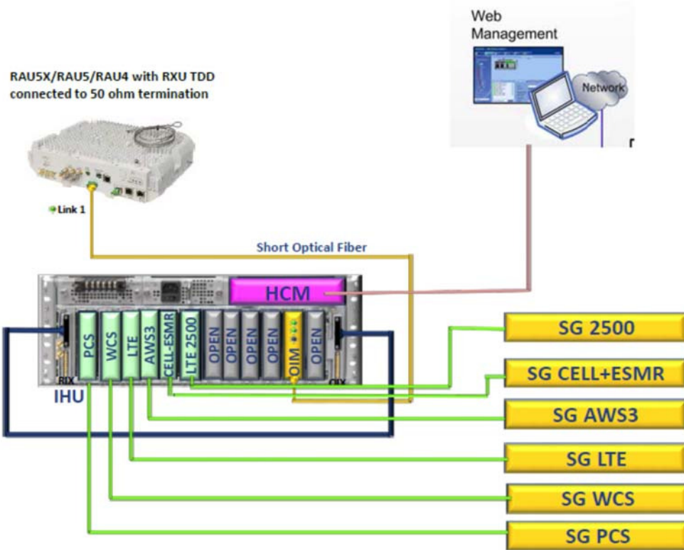
Figure 2. Radiated Test Set-Up
