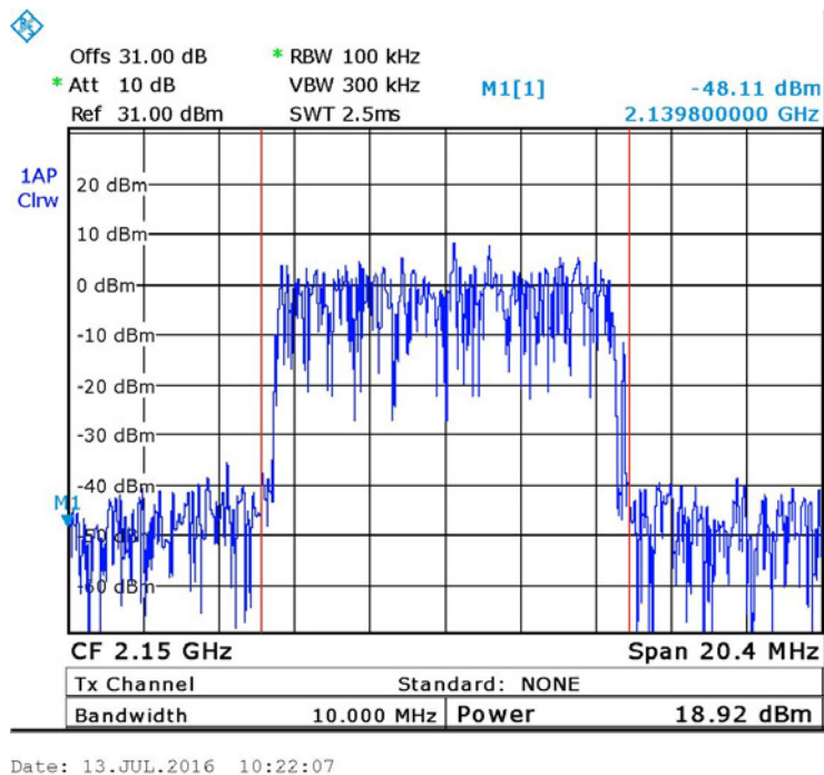
Figure 16. — LTE 64QAM (2150.00MHz)
