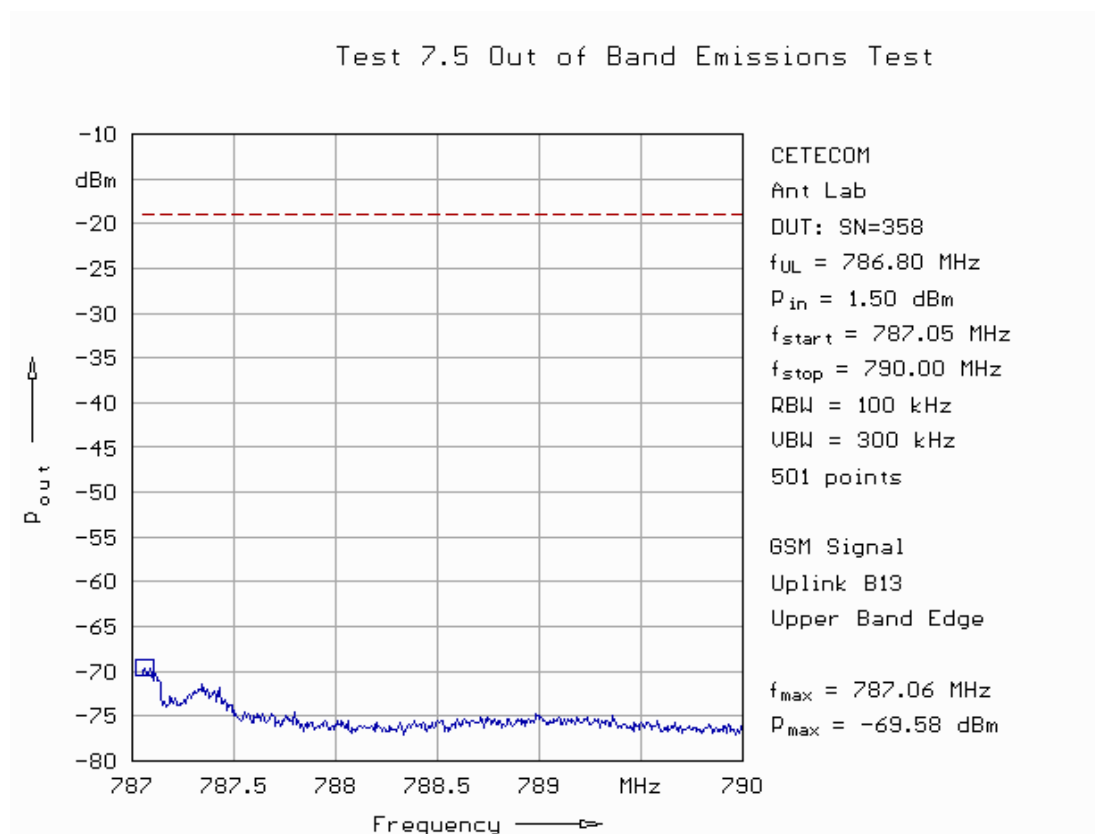
Fig. 69: Out-of-band emissions in uplink in band 13 applying a GSM signal for the upper band edge.
