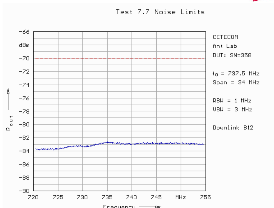
Fig. 177: Noise limits in downlink in band 12 (power off mode).
