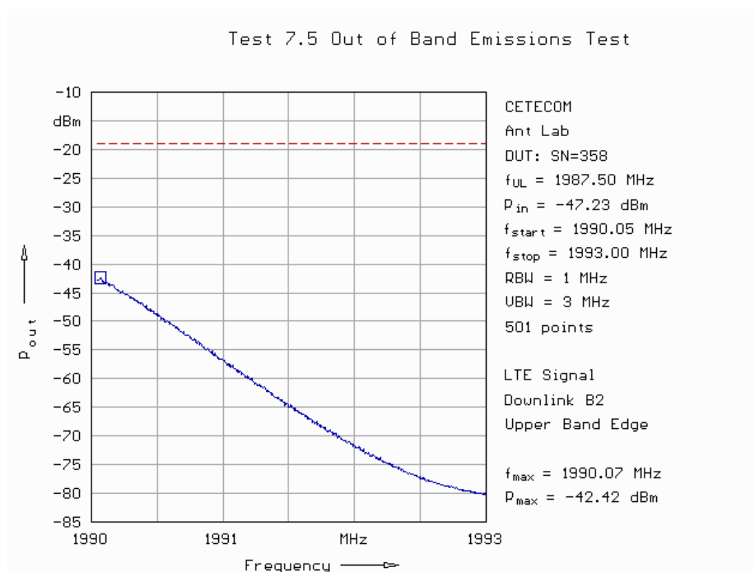
Fig. 91: Out-of-band emissions in downlink in band 2 applying a LTE signal for the upper band edge.
