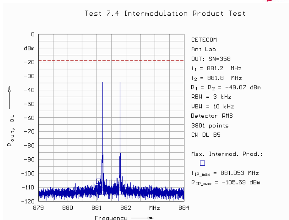
Fig. 50: Intermodulation test in downlink in band 5 at AGC.
