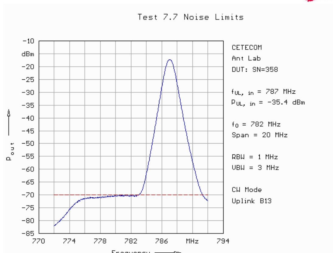
Fig. 173: Noise limits in uplink in band 13 (signal at upper band edge).
