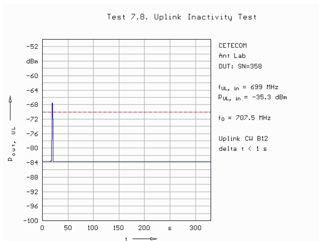
Fig. 198: Uplink inactivity test in band 12.
