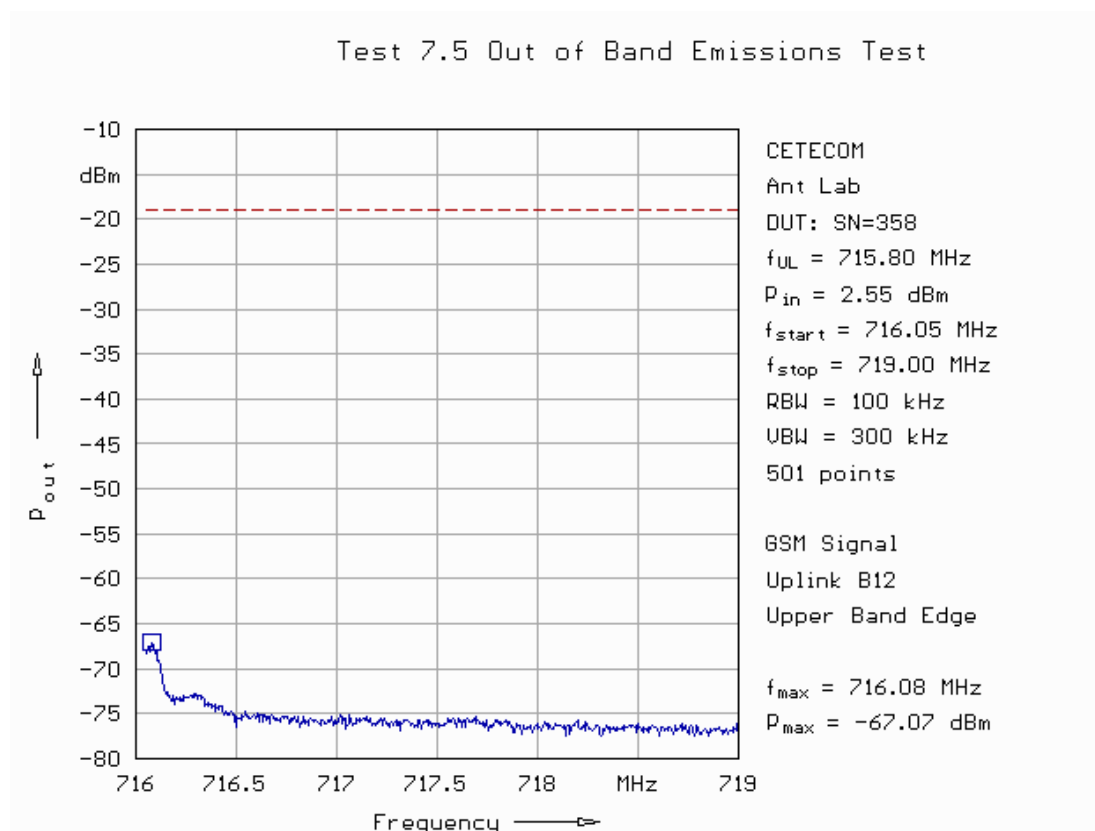
Fig. 67: Out-of-band emissions in uplink in band 12 applying a GSM signal for the upper band edge.
