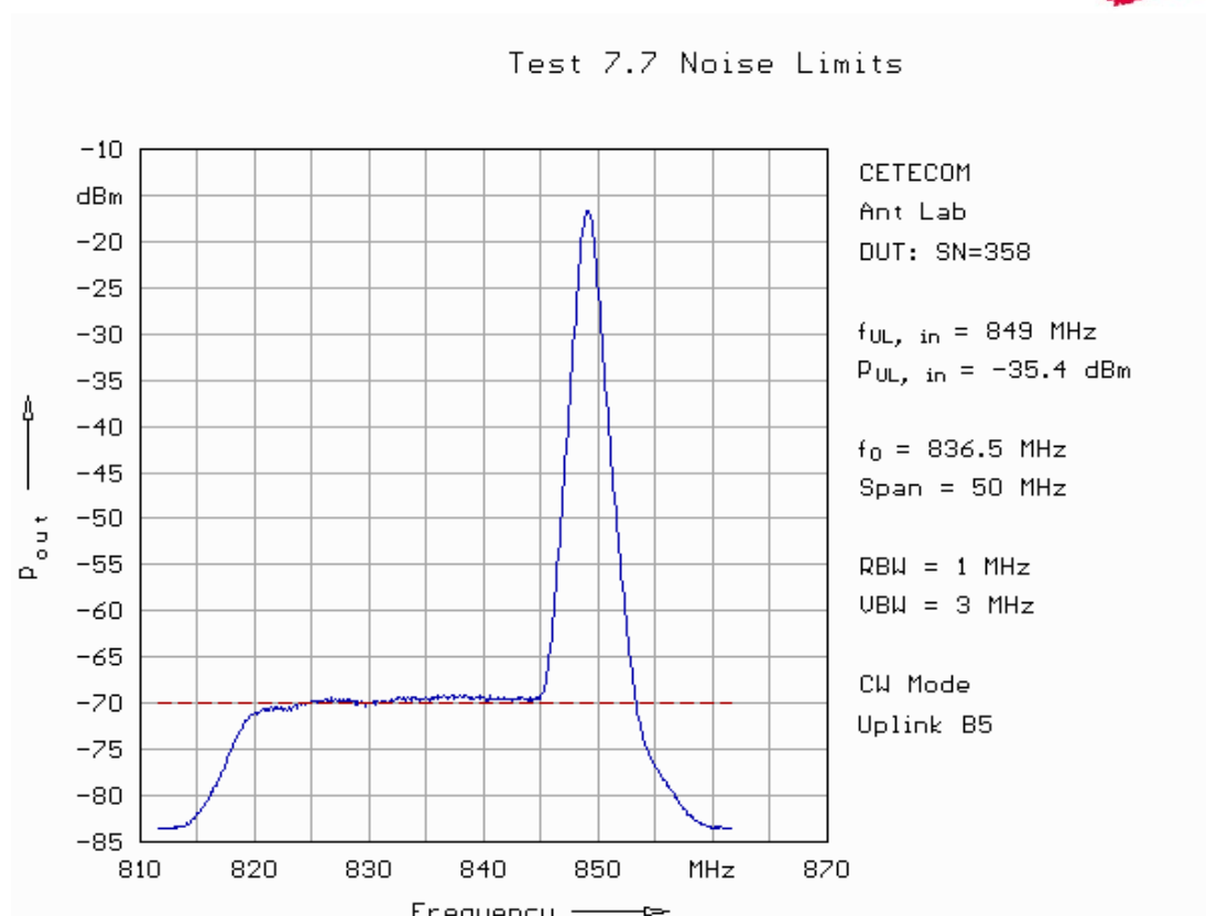
Fig. 167: Noise limits in uplink in band 5 (signal at upper band edge).
