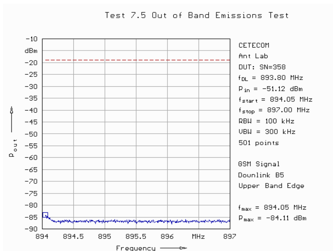
Fig. 75: Out-of-band emissions in downlink in band 5 applying a GSM signal for the upper band edge.
