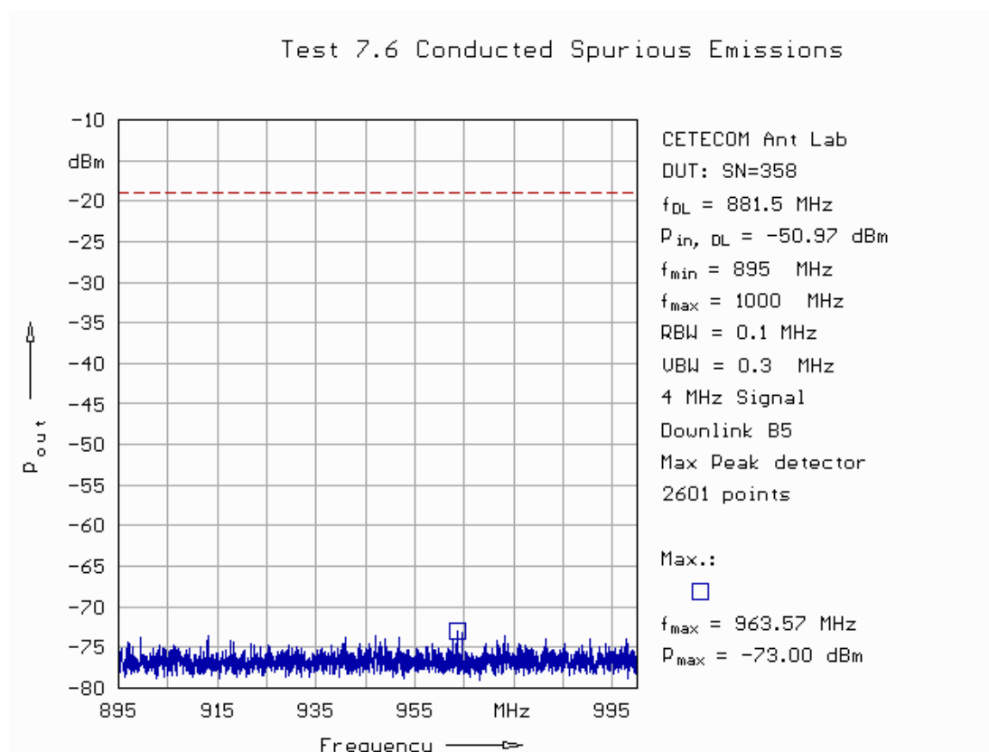
Fig. 146: Conducted spurious emissions in downlink in band 5 applying a 4 MHz signal (895 MHz – 1 GHz).
