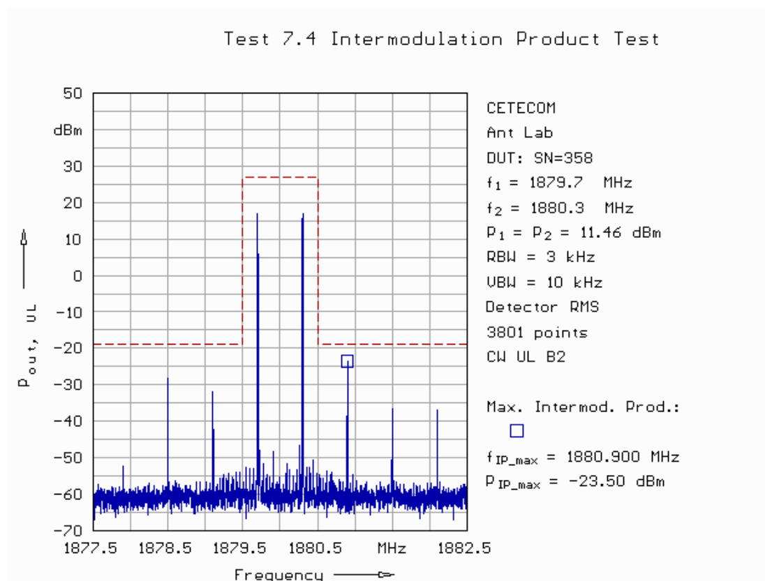
Fig. 37: Intermodulation test in uplink in band 2 at AGC plus 10 dB.
