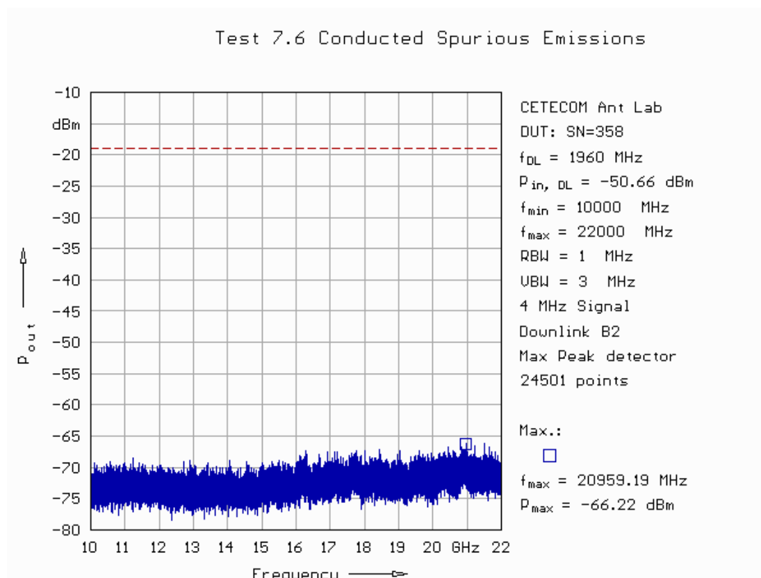
Fig. 140: Conducted spurious emissions in downlink in band 2 applying a 4 MHz signal (10 GHz – 22 GHz).
