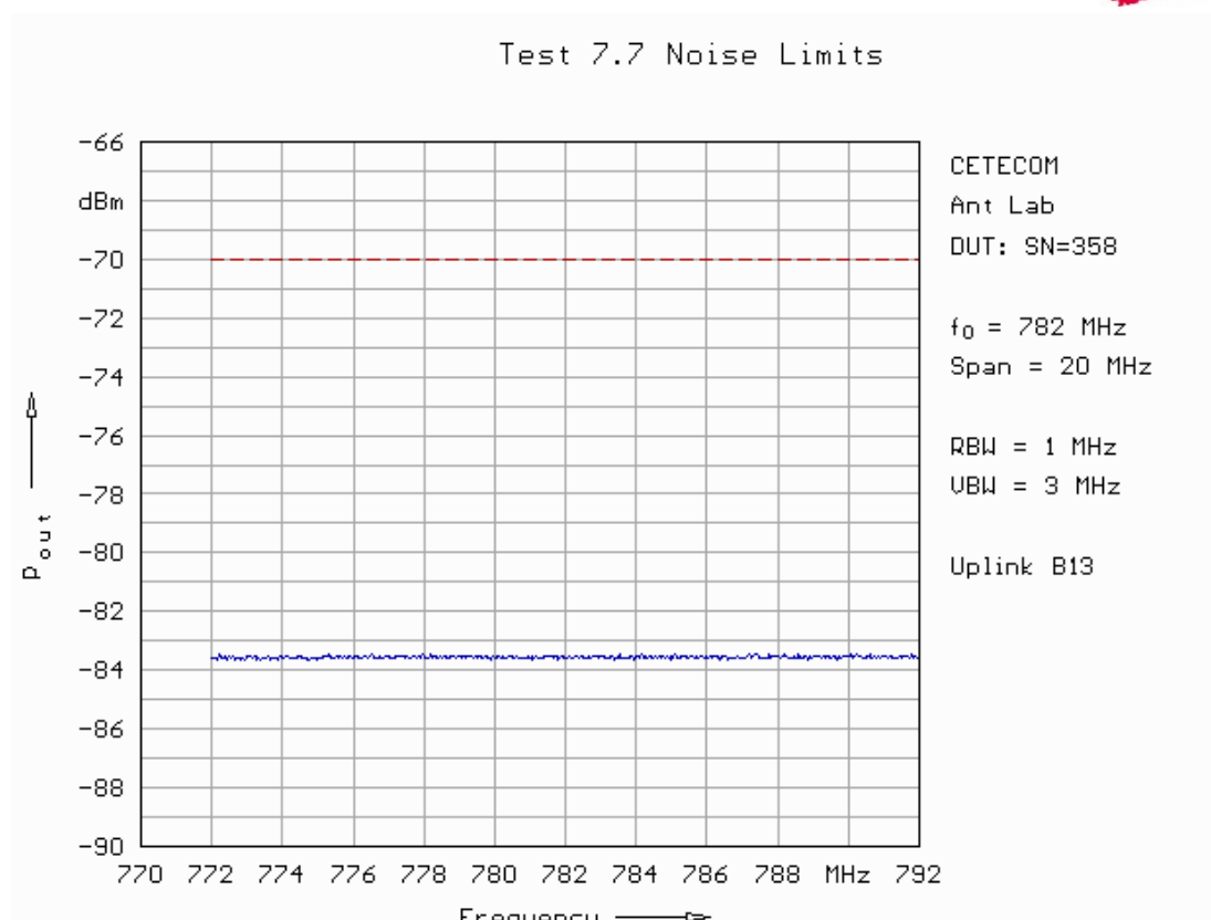
Fig. 171: Noise limits in uplink in band 13 (power off mode).
