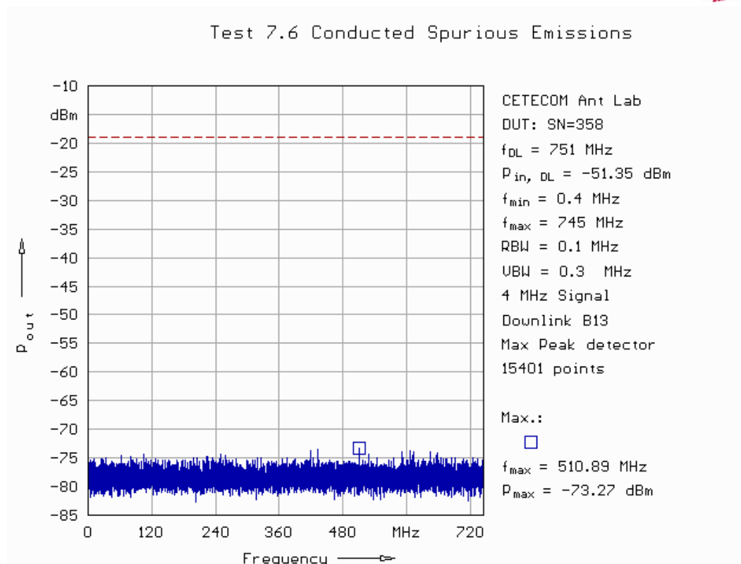
Fig. 151: Conducted spurious emissions in downlink in band 13 applying a 4 MHz signal (0.4 MHz – 745 MHz).
