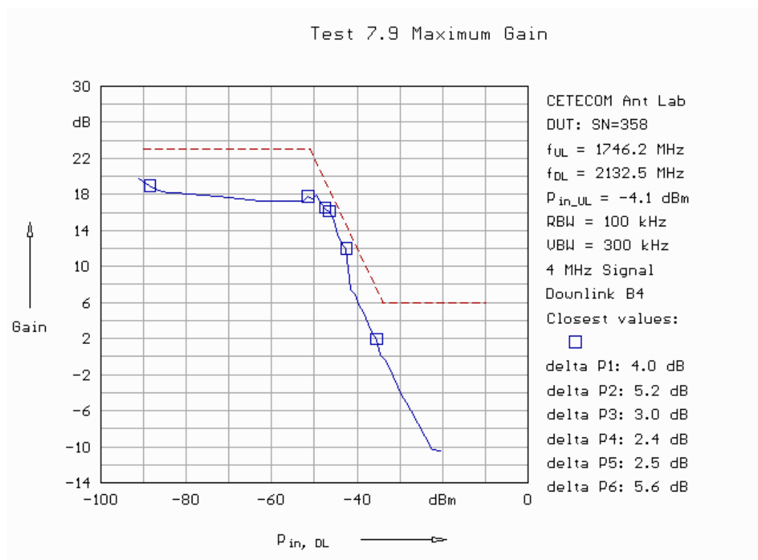
Fig. 205: Variable RSSI dependent downlink gain in band 4.
