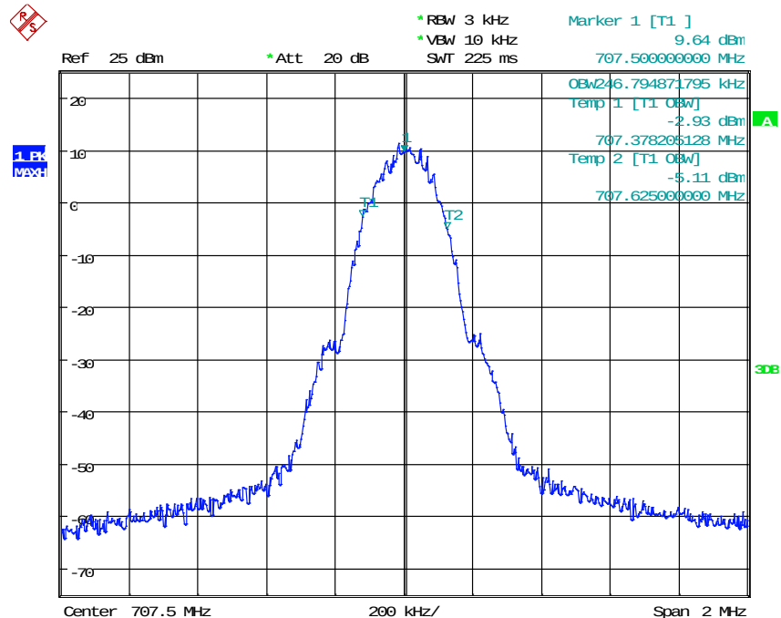
Fig. 231: Occupied bandwidth for GSM signal when using a through in band 12 uplink.
