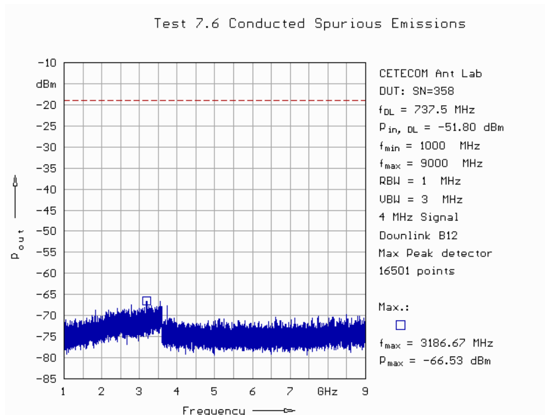
Fig. 150: Conducted spurious emissions in downlink in band 12 applying a 4 MHz signal (1 GHz – 9 GHz).
