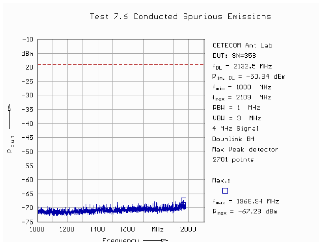
Fig. 142: Conducted spurious emissions in downlink in band 4 applying a 4 MHz signal (1 GHz – 2109 MHz).
