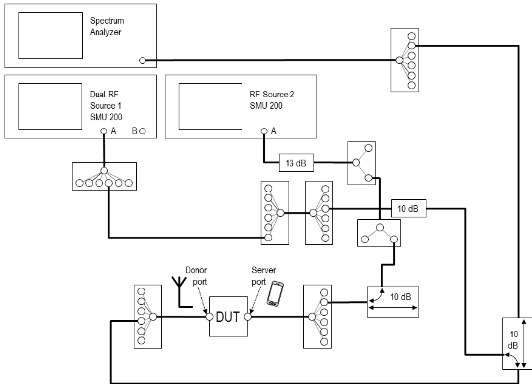
Fig. 157: Set up for the maximum transmitter noise power level test in uplink.
