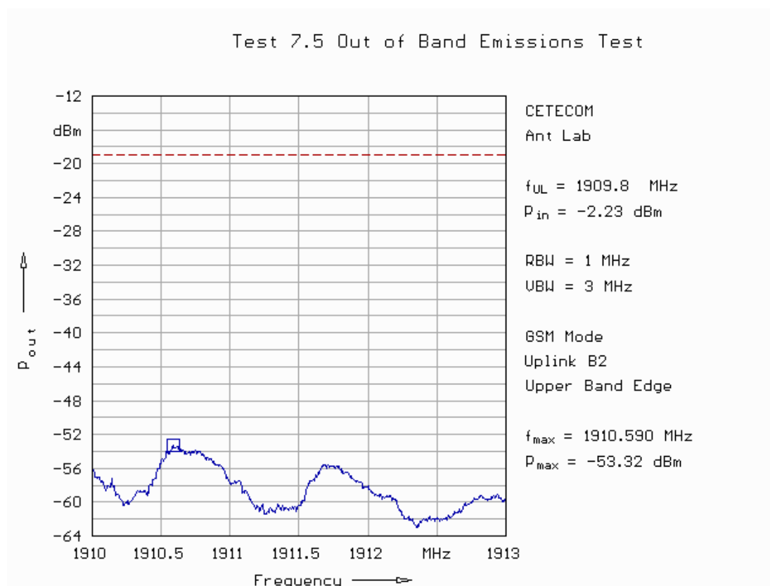
Fig. 61: Out-of-band emissions in uplink in band 2 applying a GSM signal for the upper band edge.
