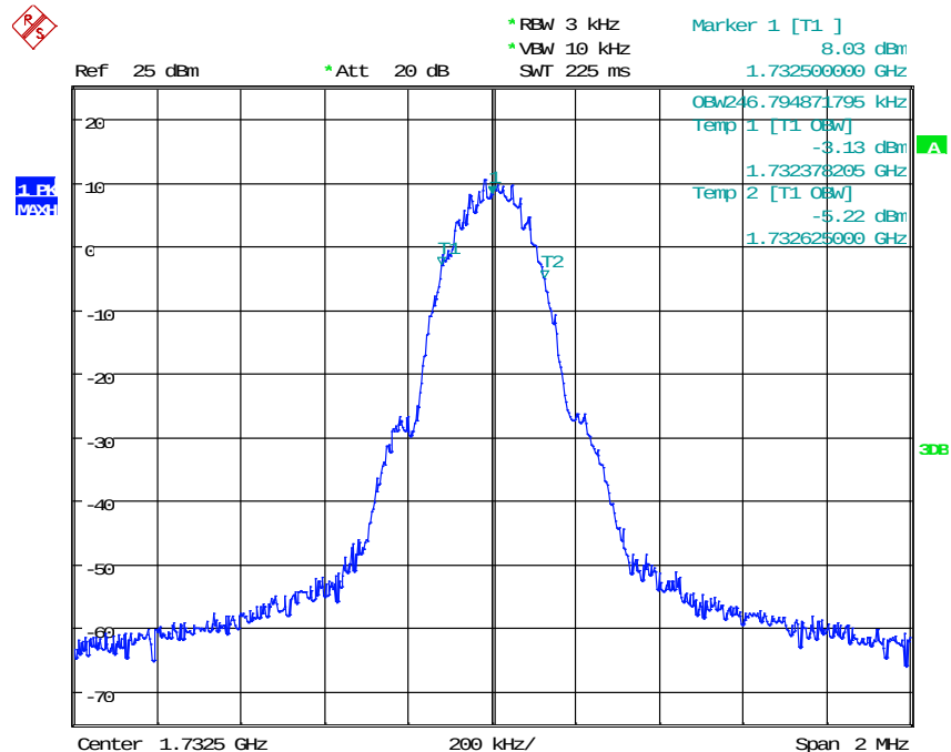
Fig. 223: Occupied bandwidth for GSM signal when using a through in band 4 uplink.
