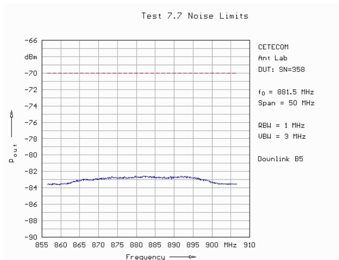
Fig. 176: Noise limits in downlink in band 5 (power off mode).
