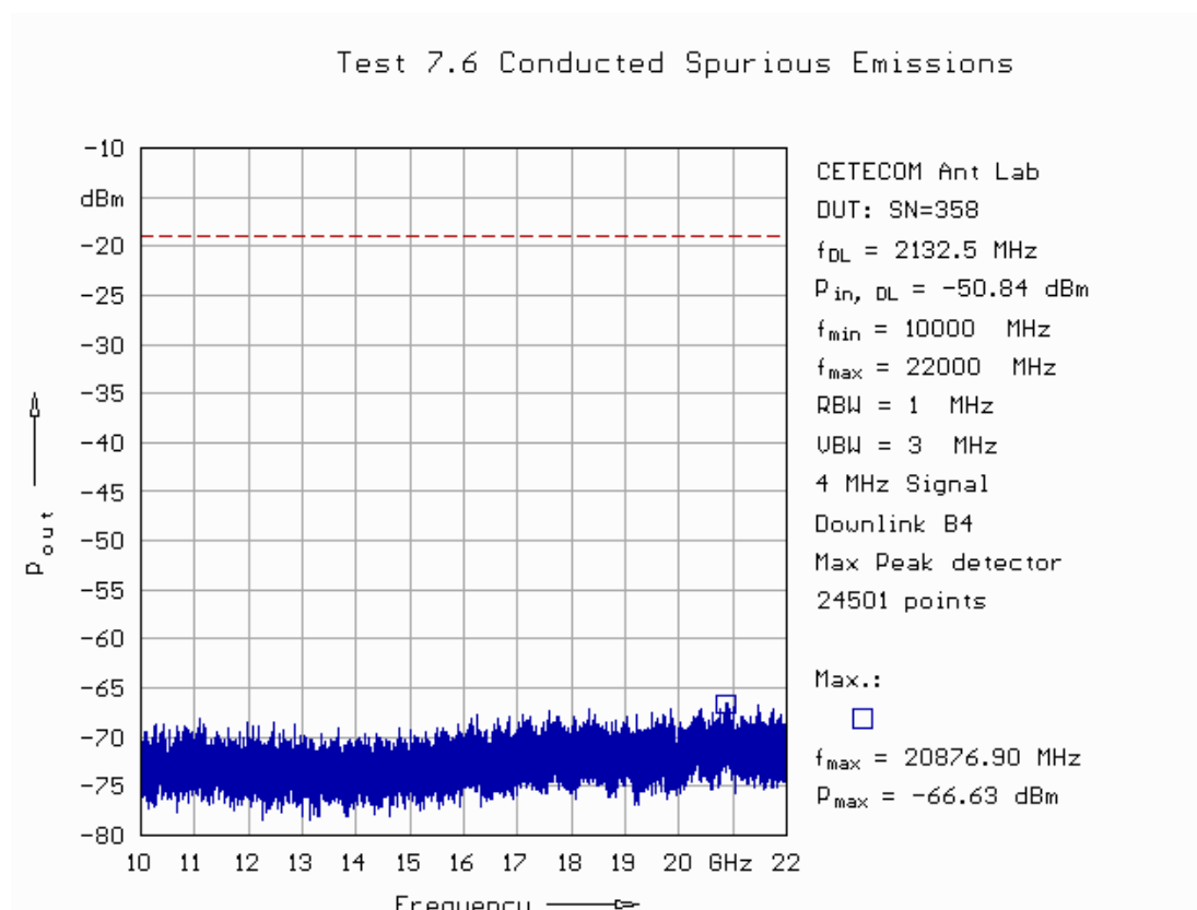
Fig. 144: Conducted spurious emissions in downlink in band 4 applying a 4 MHz signal (10 GHz – 22 GHz).
