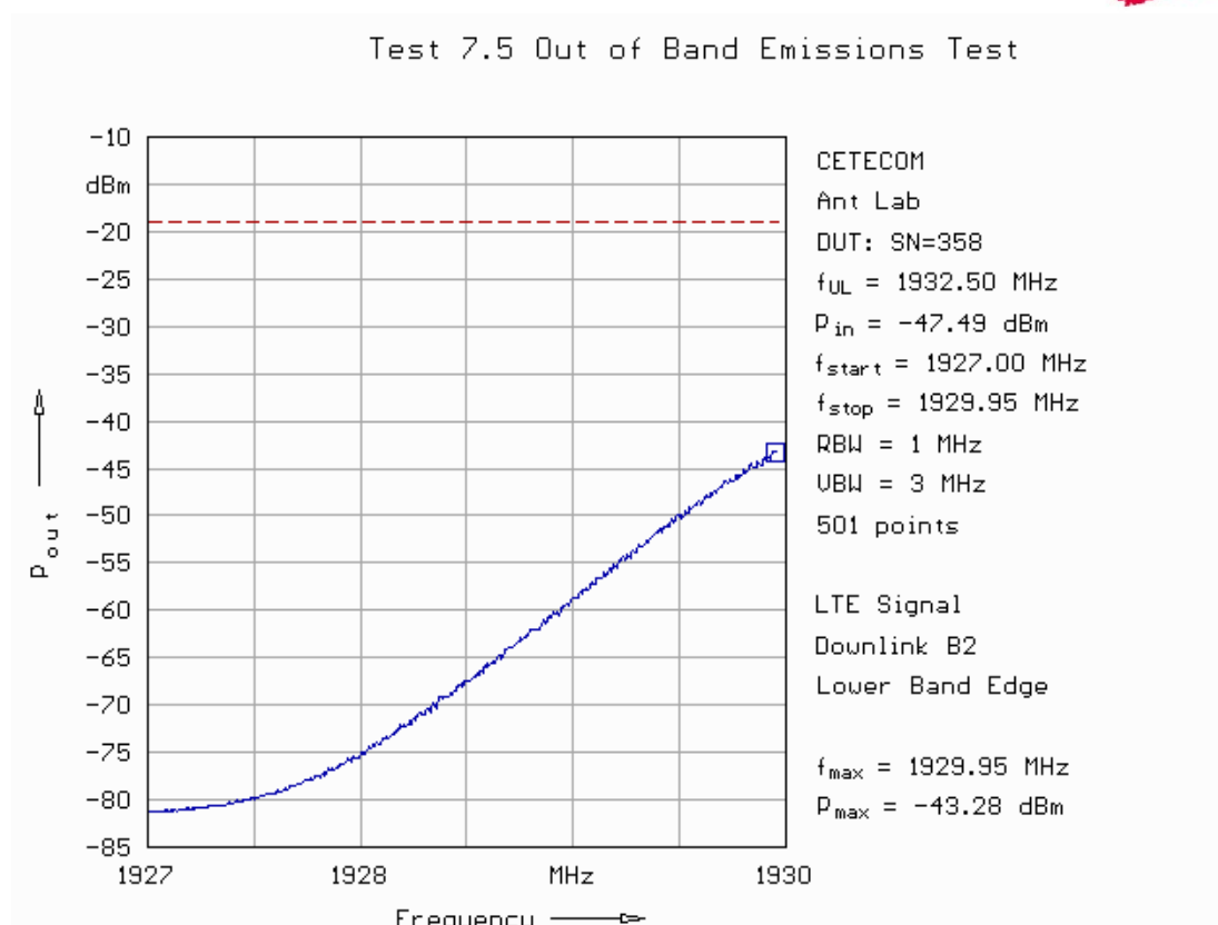
Fig. 90: Out-of-band emissions in downlink in band 2 applying a LTE signal for the lower band edge.
