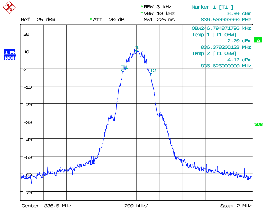
Fig. 227: Occupied bandwidth for GSM signal when using a through in band 5 uplink.
