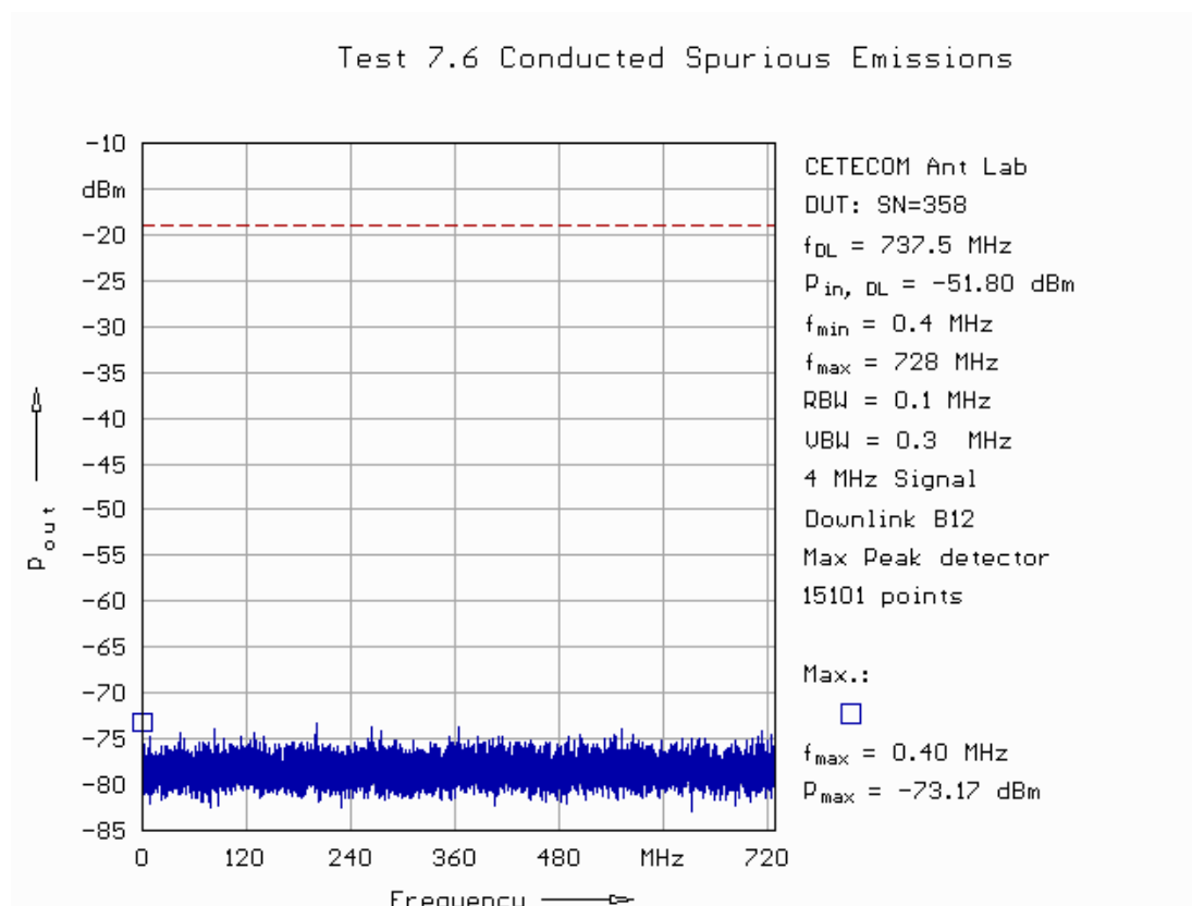
Fig. 148: Conducted spurious emissions in downlink in band 12 applying a 4 MHz signal (0.4 MHz – 728 MHz).
