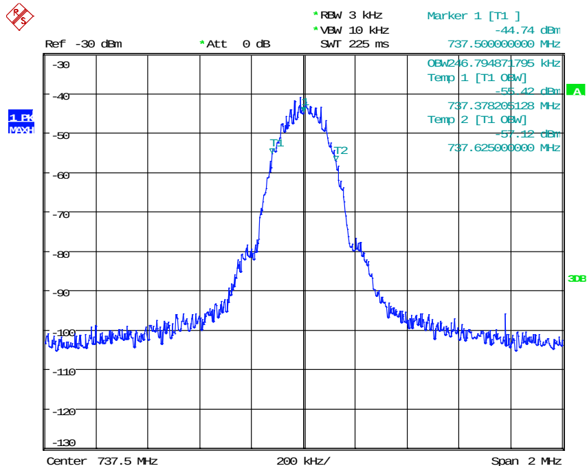
Fig. 233: Occupied bandwidth for GSM signal when using a through in band 12 downlink.
