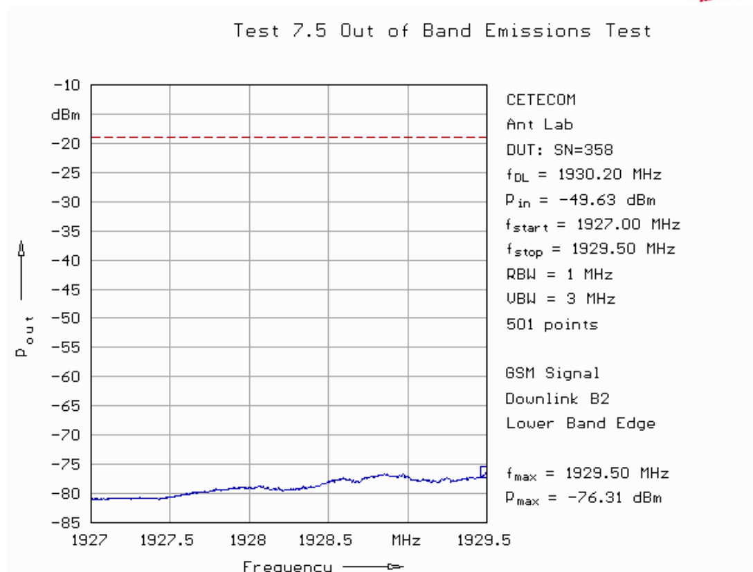
Fig. 70: Out-of-band emissions in downlink in band 2 applying a GSM signal for the lower band edge.
