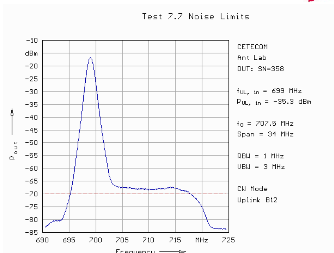
Fig. 169: Noise limits in uplink in band 12 (signal at lower band edge).
