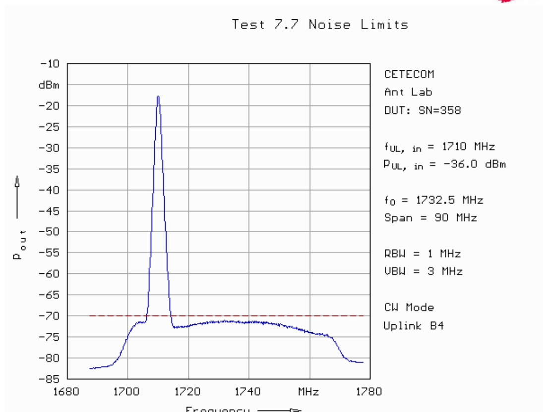
Fig. 163: Noise limits in uplink in band 4 (signal at lower band edge).
