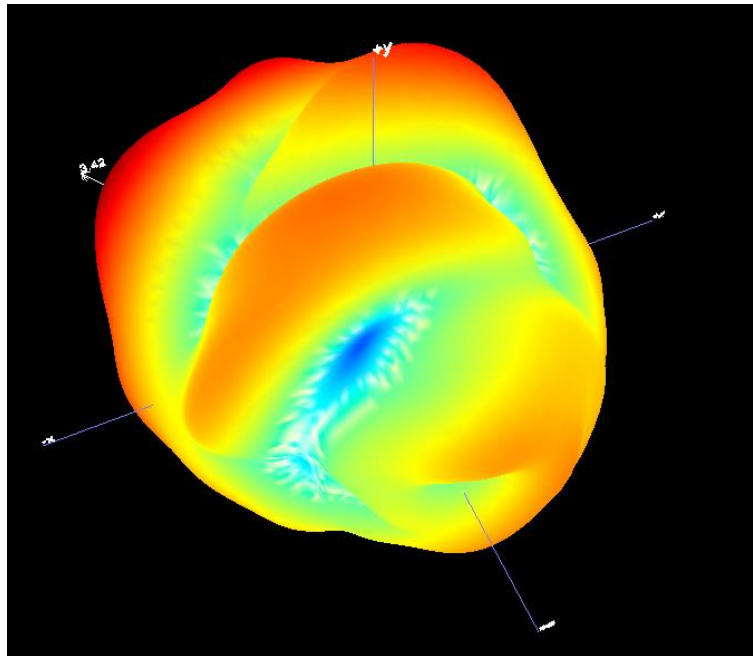
B1.1 3D Pattern for 2402MHz
