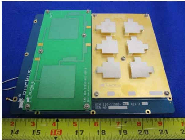
T310N Antenna Top View
