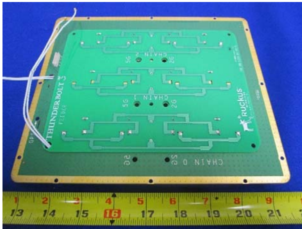
T310S Antenna Bottom View
