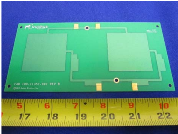
T310N Antenna Part2 Top View
