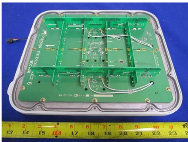
T310S Antenna Set View
