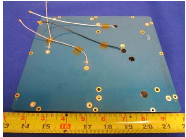
T310N Antenna Bottom View
