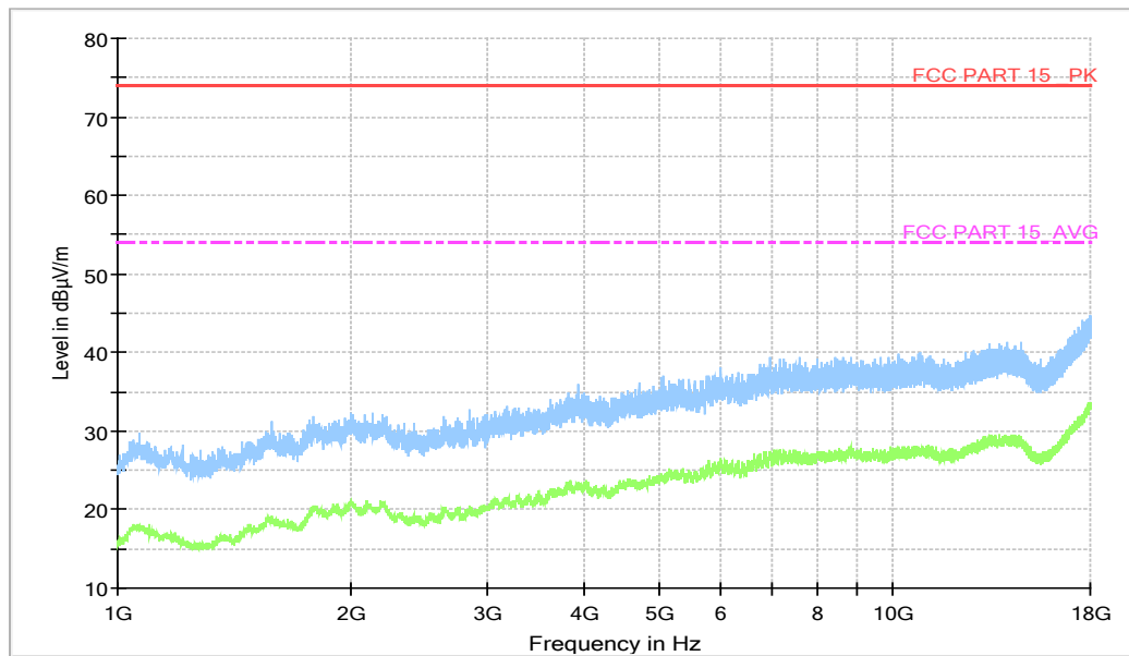
Figure A.26 Radiated Emission from 1GHz to 18GHz
