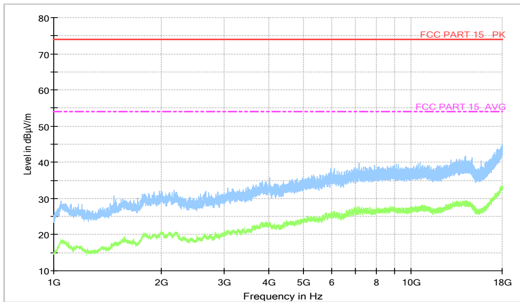
Figure A.32 Radiated Emission from 1GHz to 18GHz
