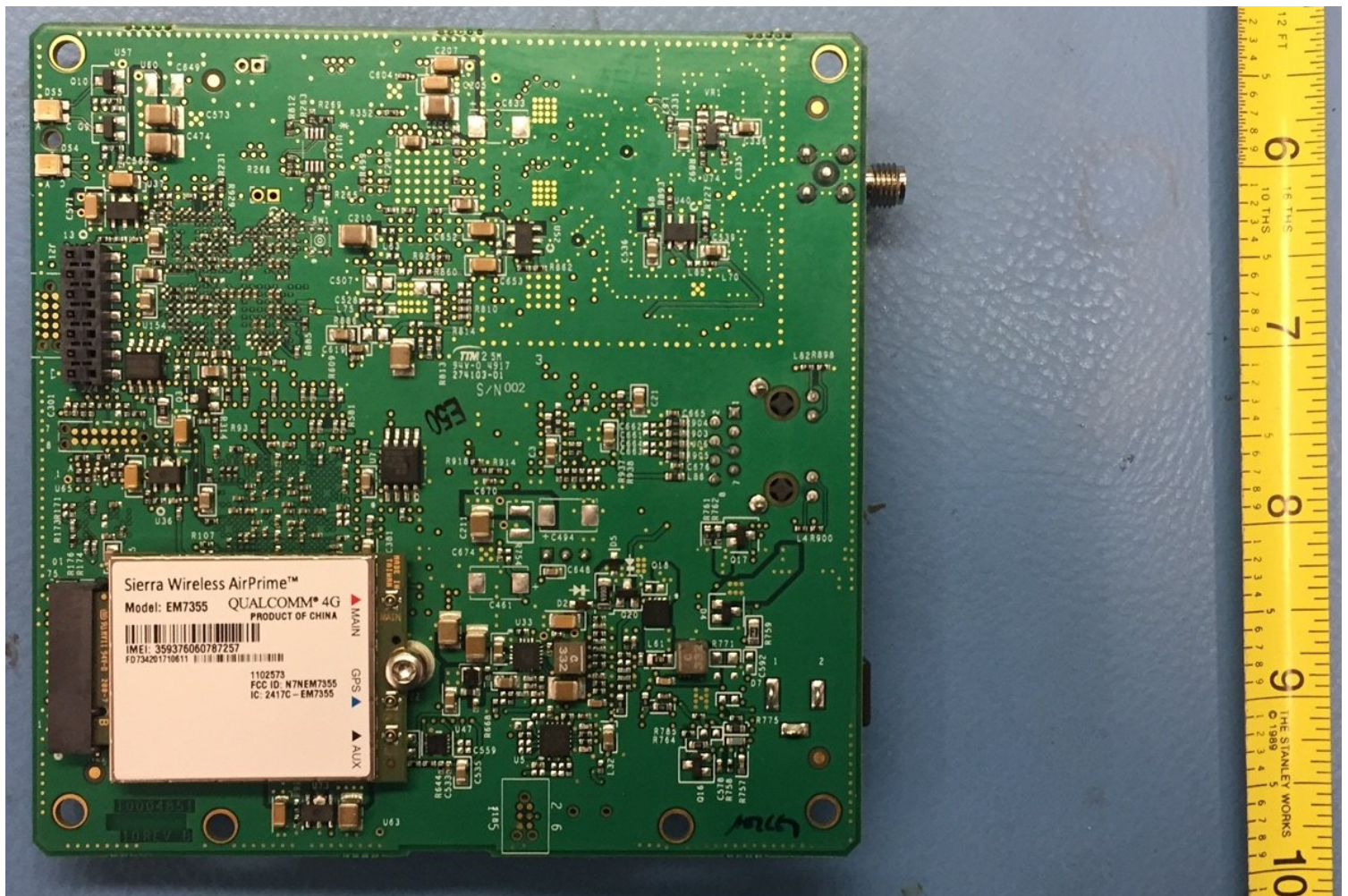
EUT PCB: Bottom View with scale
