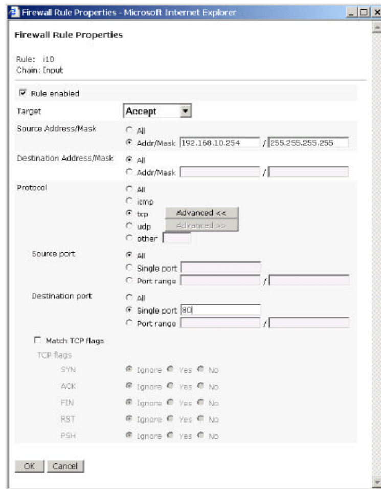
Figure 5-2 Example: Firewall rule i10
