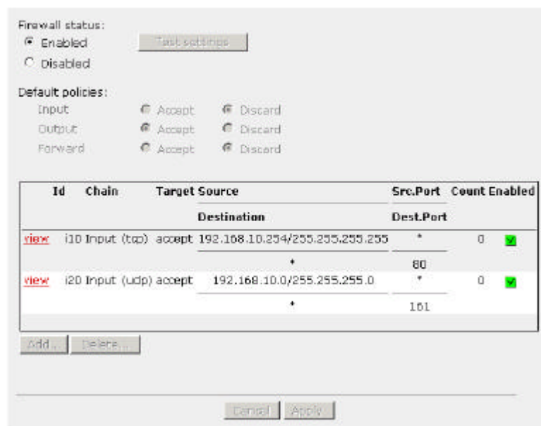
Figure 5-4 Firewall example 1
