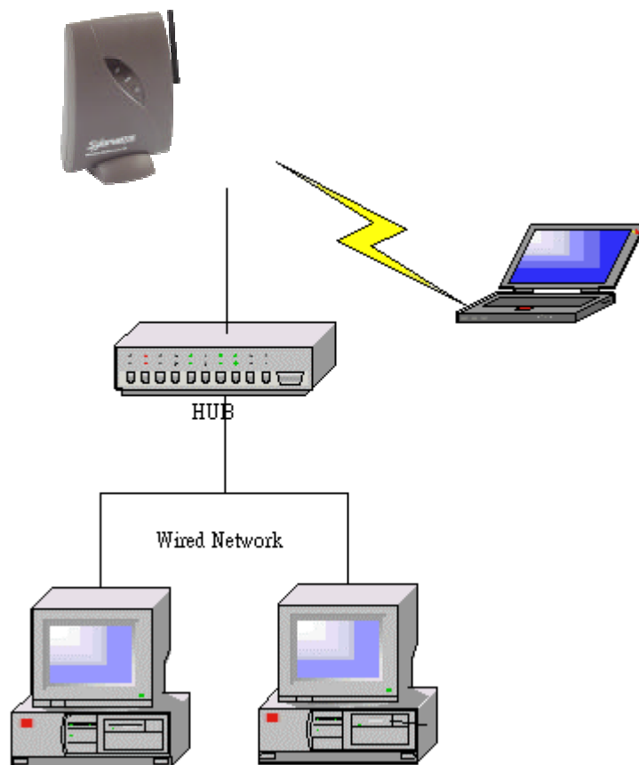
Figure 1-3 Adding an Access Point to a wired network
